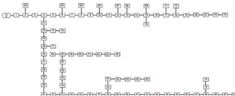
Figure 16. The topology of the test network T2.
