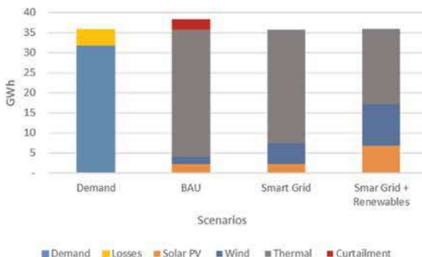
Figure 7. Scenario's energy balance.
