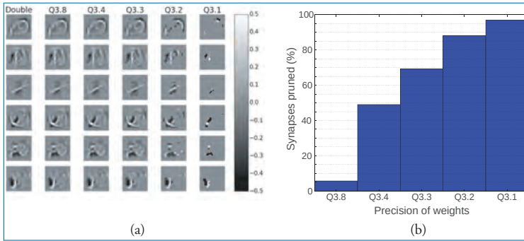
Figure 6.8. Impact of weight bit precision on the representations within a DBN. (a) The receptive fields of the first 6 neurons (rows) in the first hidden layer of the DBN with the two hidden layers. (b) Percentage of synapses from all layers that are set to zero due to the reduction in bit precision for the fractional part. Figure by Stomatias [241] with minor modifications.
