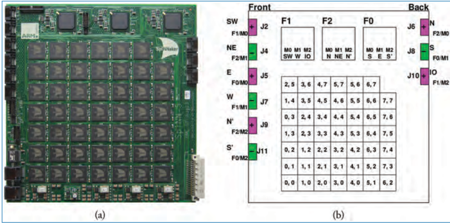
Figure 3.5. SpiNN-5: SpiNNaker production board.
