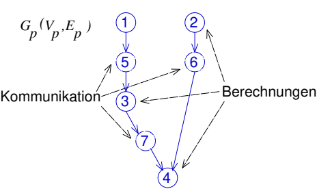
Abb. 6.32 DOL Problem-Graph
