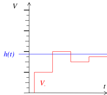
Abb. 3.12 Sukzessive Approximation
