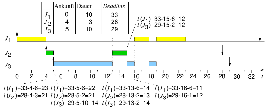
Abb. 6.8 Least laxity-Schedule
