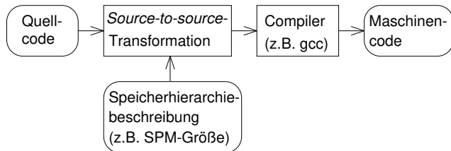
Abb. 7.12 Source-to-source-Transformation
