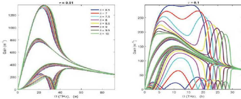
Figure 3. MI gain spectra g ( m^{-1} ) as a function of the frequency \Omega (THz) for different values of \delta in mixed GVD. (a) for \tau = 0.01ps , (b) for \tau = 0.1ps .
