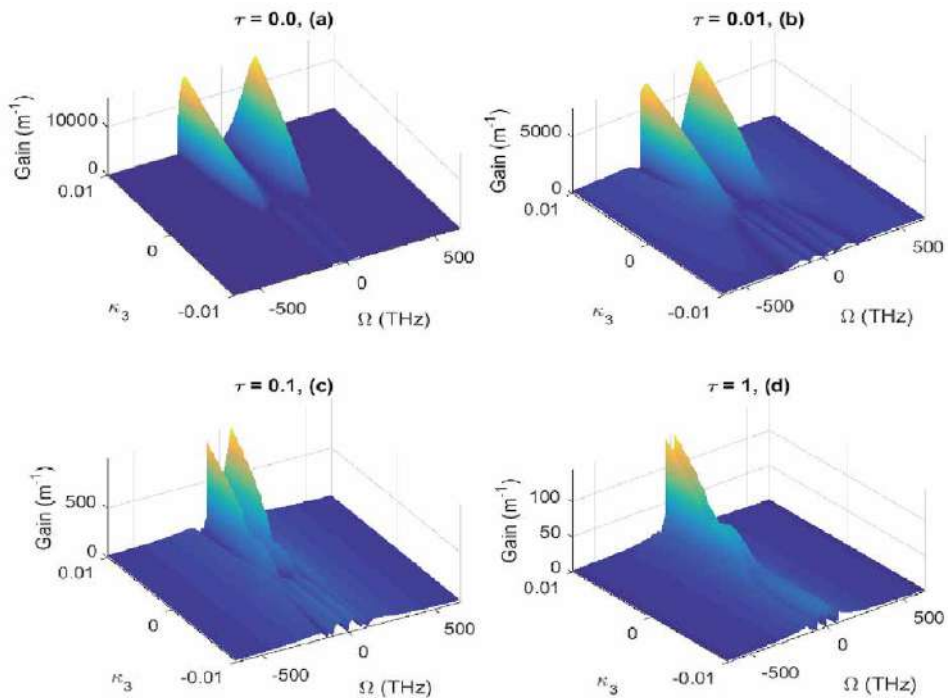
Figure 15. MI gain spectra g ( m^{-1} ) as a function of the frequency \Omega (THz) and the nonlinear parameter \kappa_3 in the case of mixed GVD for null GVM ( \delta = 0 ). (a) \tau = 0.0ps , (b) \tau = 0.01ps , (c) \tau = 0.1ps , (d) \tau = 1ps .
