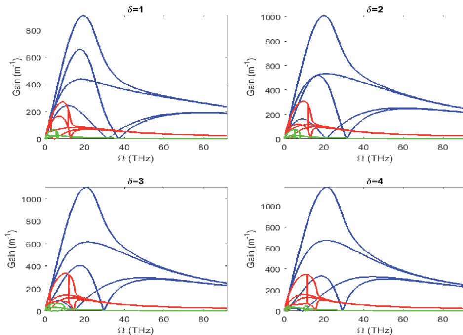
Figure 2. MI gain spectra g ( m^{-1} ) as a function of the frequency \Omega (THz) for non null GVM and nonlinear response time.
