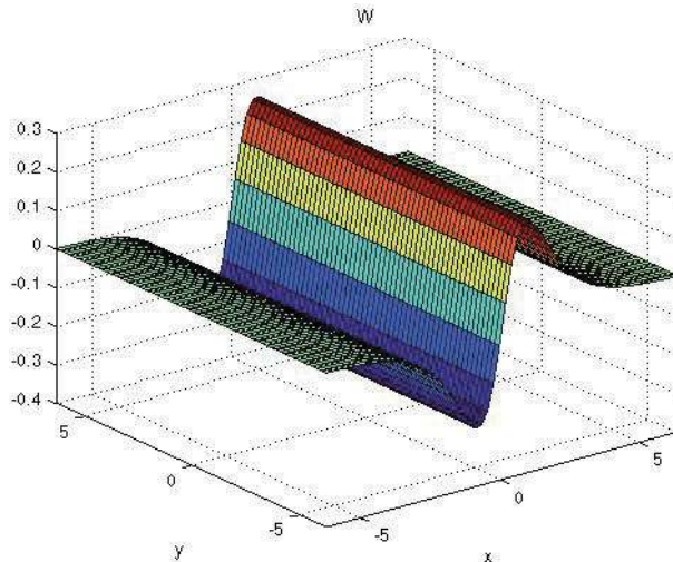
Figure 3. Profile of potential W(x) along the optical lattice.
