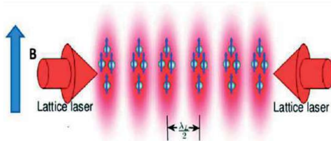
Figure 1. Schematic diagram of spinor BECs confined in a one-dimensional optical lattice. A strong static magnetic field B is applied to polarize the ground-state spin orientations of the atomic chain along the quantized z -axis.
