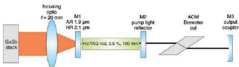
Figure 4. Resonator of the AO Q-switched Ho(0.5%):YAG laser formed by mirror M 1 and mirror M 3 (output coupler). [Reprinted/Adapted] With permission from Ref. [34] © The Optical Society.
