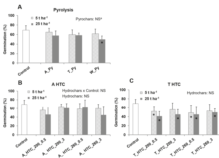
Figure 1. Germination rate (%) of Lolium perenne in: (A) Control and pyrochars-amended pots, (B) Control and pots amended with hydrochars derived from A_SS and (C) Control and pots amended with hydrochars derived from T_SS. Hydrochars were produced from primary (A_) and secondary (T_) sewage sludges at 200 °C (A_HTC_200) and 260 °C (A_HTC_260) for 0.5 and 3 h (A_HTC_200_0.5, A_HTC_200_3, respectively). Pyrochars were produced from primary (A_) and secondary (T_) sewage sludges (Py). NS: no significance. Asterisks inside the bars show significant differences to the control according to the t-test.
