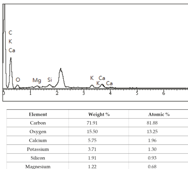
Figure 6. Energy-dispersive X-ray spectrometry (EDS) analyses of optimal biochar product (i.e., DMC-900).
