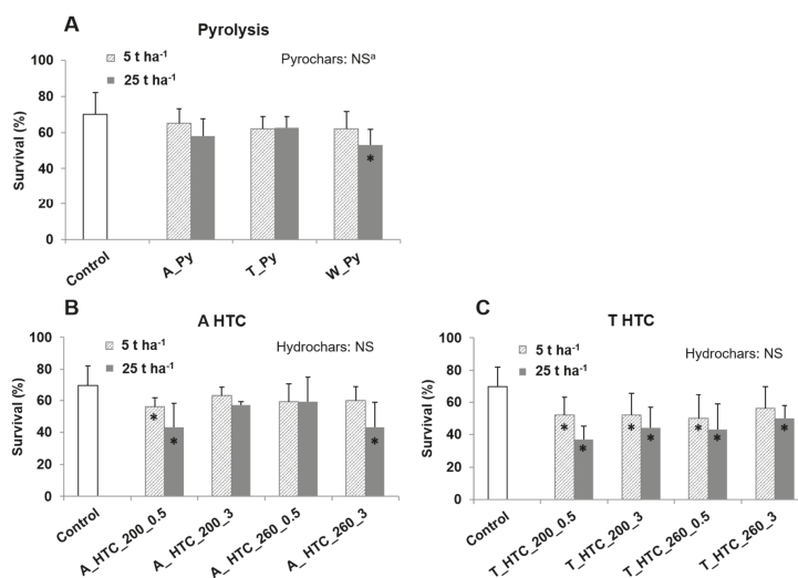
Figure 2. Survival rate (%) of Lolium perenne in: (A) Control and pyrochars-amended pots, (B) Control and pots amended with hydrochars derived from A_SS and (C) Control and pots amended with hydrochars derived from T_SS. Hydrochars were produced from primary (A_) and secondary (T_) sewage sludges at 200 °C (A_HTC_200) and 260 °C (A_HTC_260) for 0.5 and 3 h (A_HTC_200_0.5, A_HTC_200_3, respectively). Pyrochars were produced from primary (A_) and secondary (T_) sewage sludges (Py). NS: no significance. Asterisks inside the bars show significant differences to the control according to the t-test.
