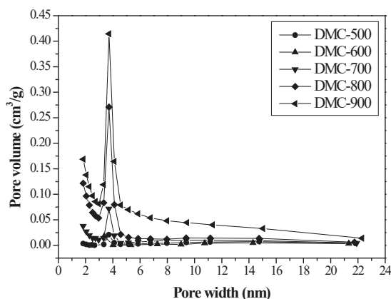
Figure 4. Pore size distributions of DMC products (i.e., DMC-500, DMC-600, DMC-700, DMC-800, and DMC-900).
