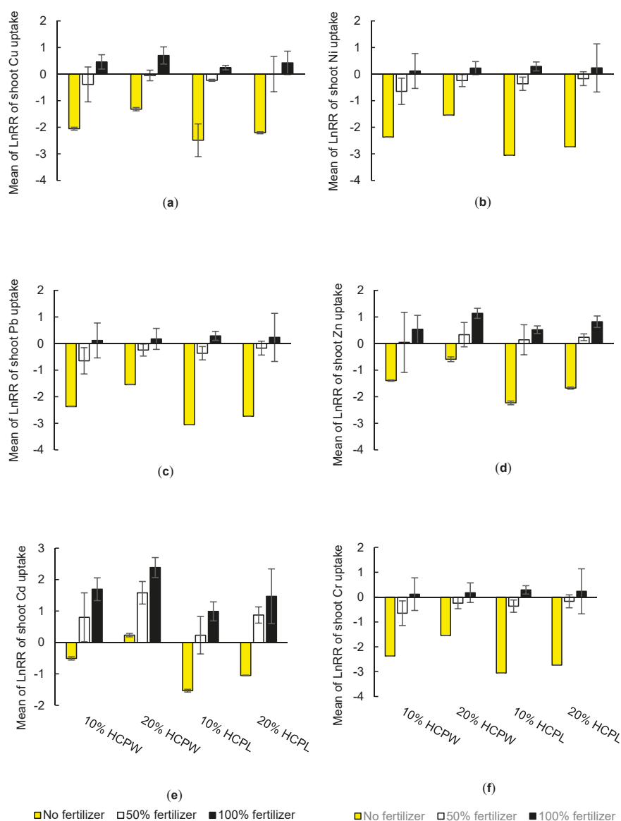
Figure 4. Mean ( \pm 95 CI, n = 3 ) natural logarithmic response ratios (standardized with the untreated fully-fertilized control) of shoot Cu (a), Ni (b), Pb (c), Zn (d), Cd (e) and Cr (f) uptake of pine tree seedlings grown in peat mixed with 10% and 20% (v/v) hydrochar powder (HCPW) and hydrochar pellet (HCPL) in unfertilized (yellow bars), half (open bars) and full fertilized (black bars) conditions. Effects of hydrochar type and application rate were considered significant, relative to controls receiving 100% fertilizer, when 95% CI did not overlap with zero in each nutritional regime.
