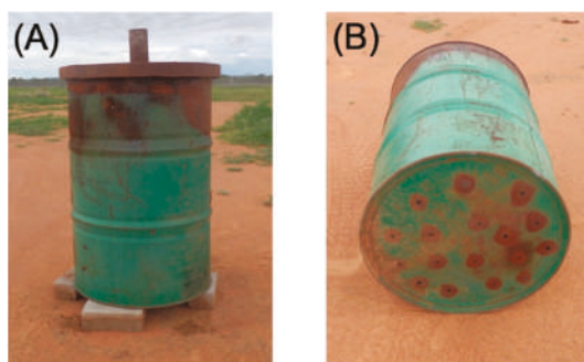
Figure 1. Jatropa fallen leaf biochar production using an oil-drum carbonizer. (A) Side view of the carbonizer. An oil drum was placed on top of bricks and covered with a custom-made lid with a funnel. (B) Bottom view of the carbonizer. Several ventilation holes were made in the bottom of the oil drum.
