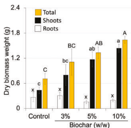
Figure 5. Effects of jatropha fallen leaf biochar application to the experimental soil on the dry biomass weight of Swiss chard plants at harvest (44 days after transplantation). Values are means \pm standard deviations of three independent plants. Sets of bars with different letters are significantly different (Holm's test, p < 0.05 ).
