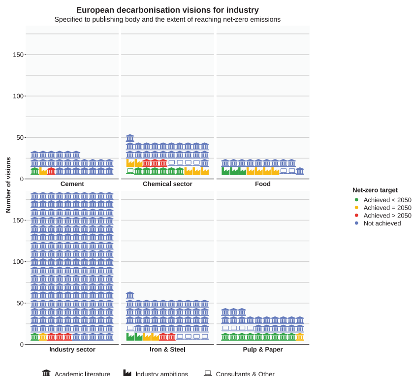
Figure 2 Overview of quantified visions for European industry decarbonisation, looking both at visions developed in academics (Greek temple) or industry (factory)
