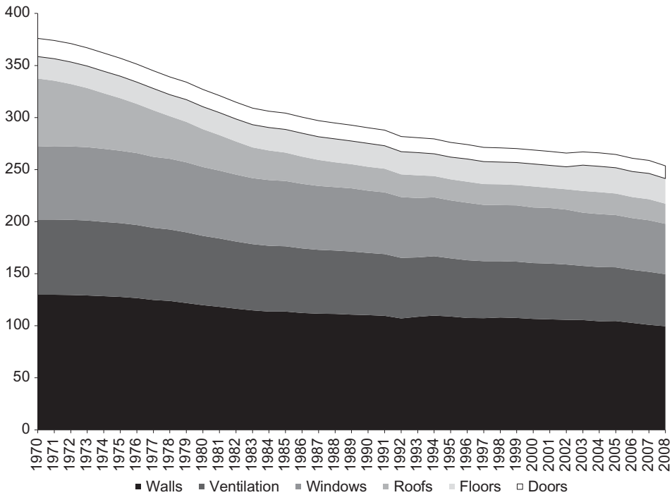
Figure 6.10 Average heat loss per dwelling in W/^{\circ}C (constructed using data from DECC (2012a))
