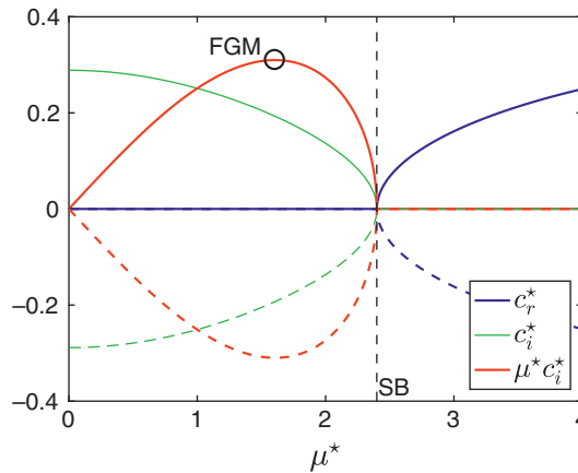
Figure 8.6 Phase speed (real = blue , imaginary = green ) and scaled growth rate \mu^* c_i^* ( red ) versus vertical length scale for the Eady model of baroclinic instability, based on (8.57). Scalings are defined by \mu^* = \mu H and c^* = c/U_z H . Annotations mark the fastest-growing mode (FGM) and the stability boundary (SB).
