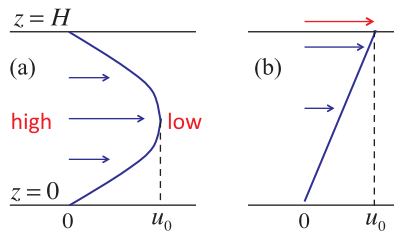
Figure 5.2 Equilibrium states in a viscous fluid. (a) Plane Poiseuille flow maintained by a uniform pressure gradient. (b) Plane Couette flow driven by a moving upper boundary.
