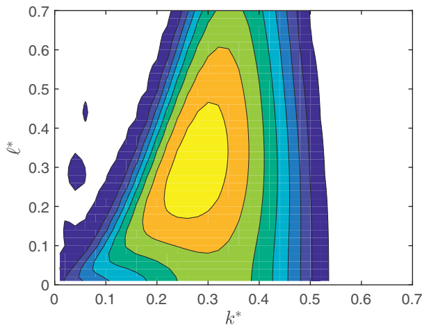
Figure 6.7 Holmboe instability growth rate versus scaled wavenumbers k^* and \ell^* for Re = 200 and Ri_0 = 0.3 . The contour interval is 0.002, starting at zero. The fastest-growing mode is oblique.
