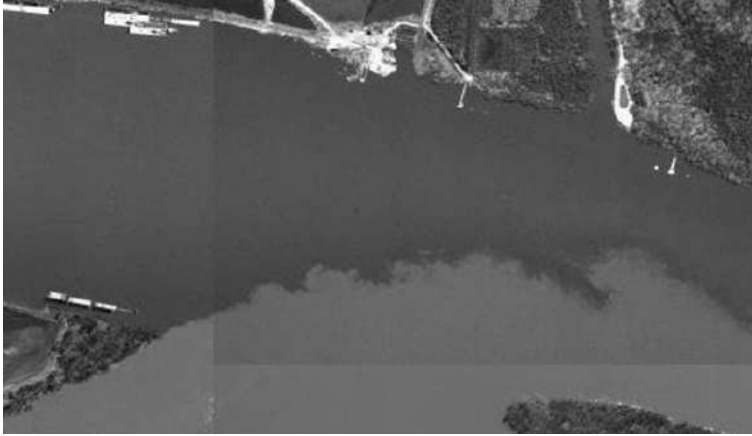
Figure 4.15 Confluence of the silty Missouri and clearer Mississippi rivers near St. Louis, MO, showing spatially growing instability. Image courtesy United States Geological Survey (USGS).
