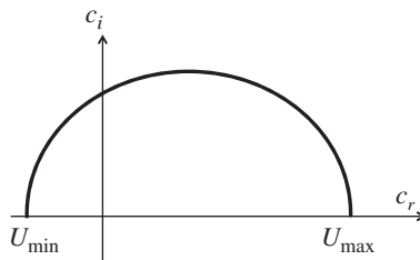
Figure 4.14 Howard's semicircle on the complex c -plane, bounded by the extremal values of the mean velocity. The phase speed of an unstable mode must lie within the semicircle (Howard, 1961).
