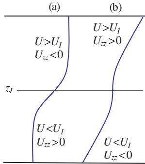
Figure 3.17 Inflectional velocity profiles. U_I = U(z_I) is the velocity at the inflection point z_I . According to the shear production theorem (which includes the Rayleigh and Fjørtoft theorems), (a) may be unstable, whereas (b) is definitely not.
