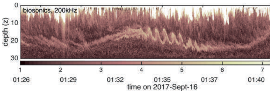
Figure 4.3 Echosounder image showing Kelvin-Helmholtz billows growing on an interfacial gravity wave off the California coast. The wave was visualized by a shipboard echosounder. Similar in principle to a medical ultrasound, it registers sound waves reflected from biota and from tiny changes in water density due to centimeter-scale turbulence. Image is courtesy of J. MacKinnon, J. Colosi, and A. Suanda.
