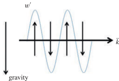
Figure 2.3 Normal mode in an inviscid, nondiffusive, uniformly stratified fluid. The wavevector is horizontal (i.e., \theta = 0 ); hence the motions are vertical. This orientation “feels” gravity most strongly: it exhibits the fastest oscillations when B_z > 0 (see equation 2.25), and the fastest exponential growth when B_z < 0 (equation 2.26).
