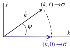
Figure 3.10 Black: wave vector (k, \ell) of an oblique mode with growth rate \sigma . Blue: wave vector (\tilde{k}, 0) of the corresponding 2D mode , with growth rate \tilde{\sigma} = \sigma / \cos \varphi \geq \sigma .
