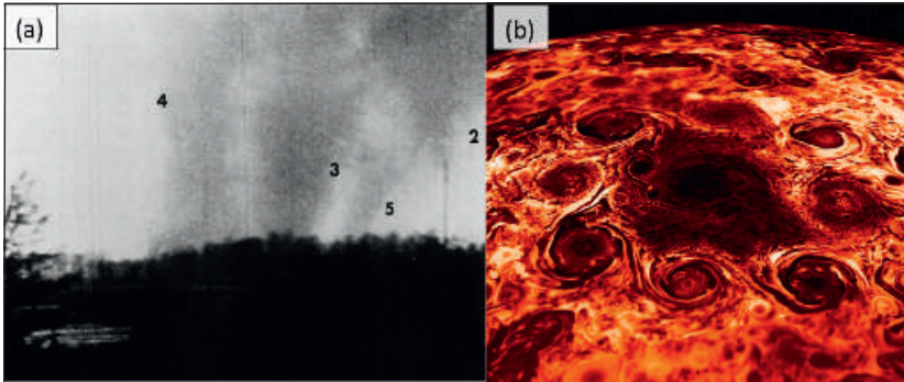
Figure 7.3 (a) Secondary vortices in a tornado suggestive of barotropic instability. Photo by W. Hubbard, WISH Indianapolis, from Snow (1978) . (b) Instability with \ell = 8 surrounding Jupiter's north polar vortex (courtesy NASA). Structures appear to be barotropic, extending as deep as 3000 km ( Adriani et al., 2018 ; Kaspi et al., 2018 ).
