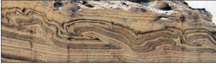
Figure 5.1 Kelvin-Helmholtz instability in paleo-earthquakes revealed in sediment deformations near the Dead Sea. The billow amplitude is \sim 1 m. These deformations can be modeled by the flow of a viscous fluid. Adapted from Heifetz et al. (2005) .
