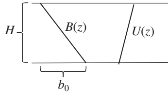
Figure 6.1 Definitions for the sheared Benard problem.
