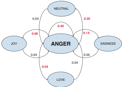
Fig. 4. Anger Markov chain. For simplicity only edges from/to ANGER are displayed
