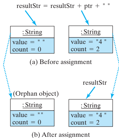
Figure 7.9: Evaluating resultStr = resultStr + ptr + " " creates an orphan object that must be garbage collected.
