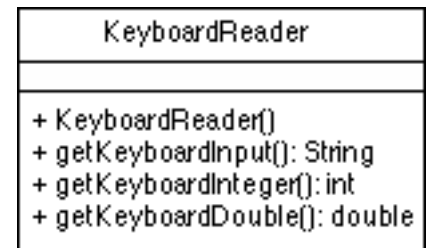
Figure 2.27: A UML class diagram of the KeyboardReader class.
