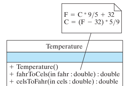
Figure 5.4: The Temperature class. Note that static elements are underlined in UML. (NEEDS REVISION)
