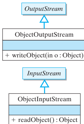
Figure 11.26: Classes used for performing I/O on objects.
