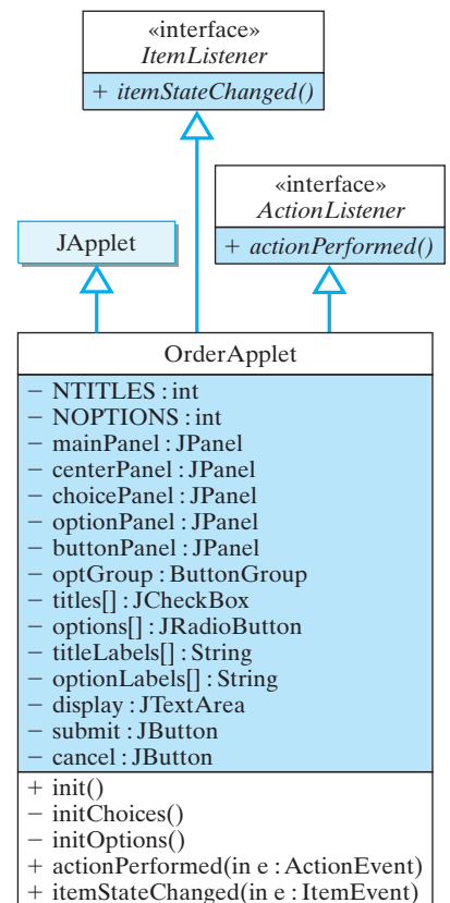
Figure 13.29: The OrderApplet makes extensive use of GUI components.
