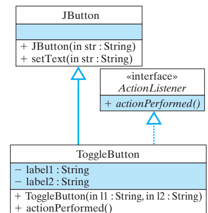
Figure 8.8: A ToggleButton is a JButton with two labels.
