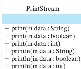
Figure 1.13: A UML class diagram of the PrintStream class.
