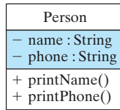
Figure 1.16: The Person class.
