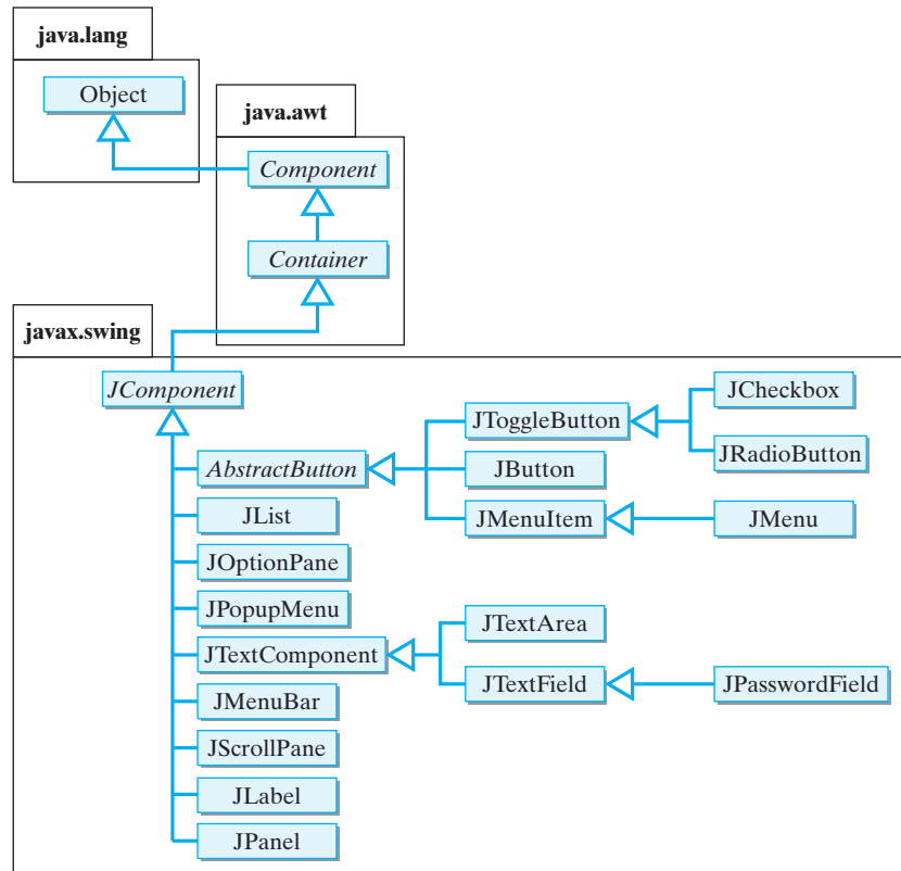
Figure 13.2: Swing classes, part 2: Swing GUI components are derived from the JComponent class.
