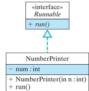
Figure 14.5: Any object that implements the Runnable interface can be run as a separate thread.
