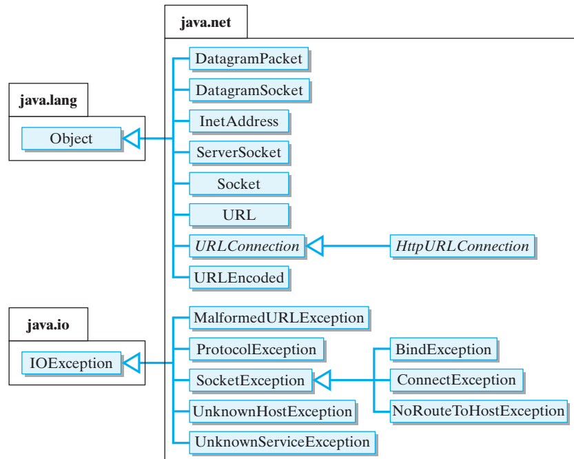
Figure 15.7: The java.net package.
