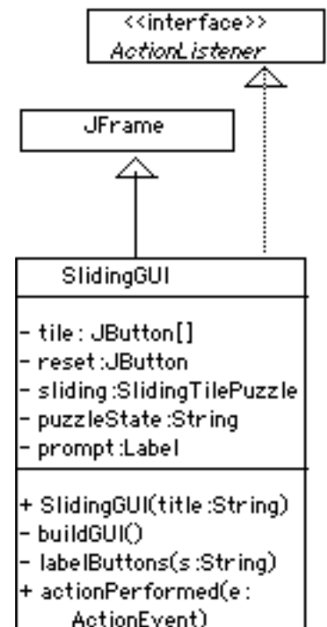
Figure 9.39: The SlidingGUI class.
