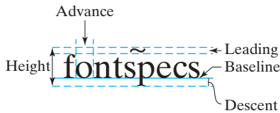
Figure 7.20: An illustration of the various font measurements.
