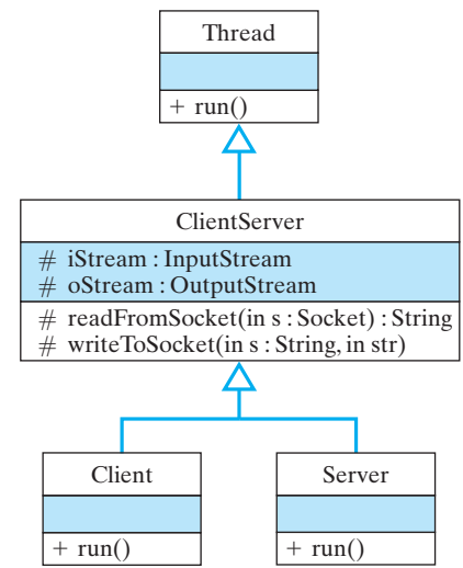
Figure 15.25: Overall design of a client/server application.
