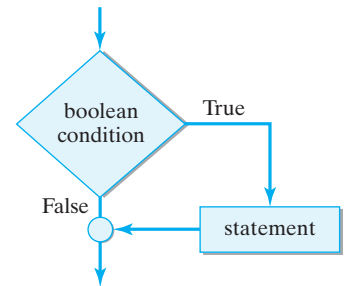
Figure 3.11: Flowchart of the if statement. Diamond-shaped symbols at the branch points contain boolean expressions. Rectangular symbols can only contain executable statements. Circles act simply as connectors, to connect two or more paths.
