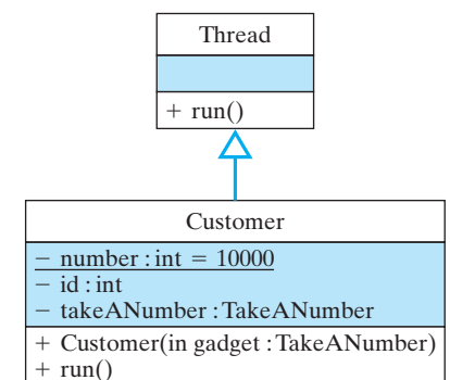
Figure 14.20: The Customer thread.
