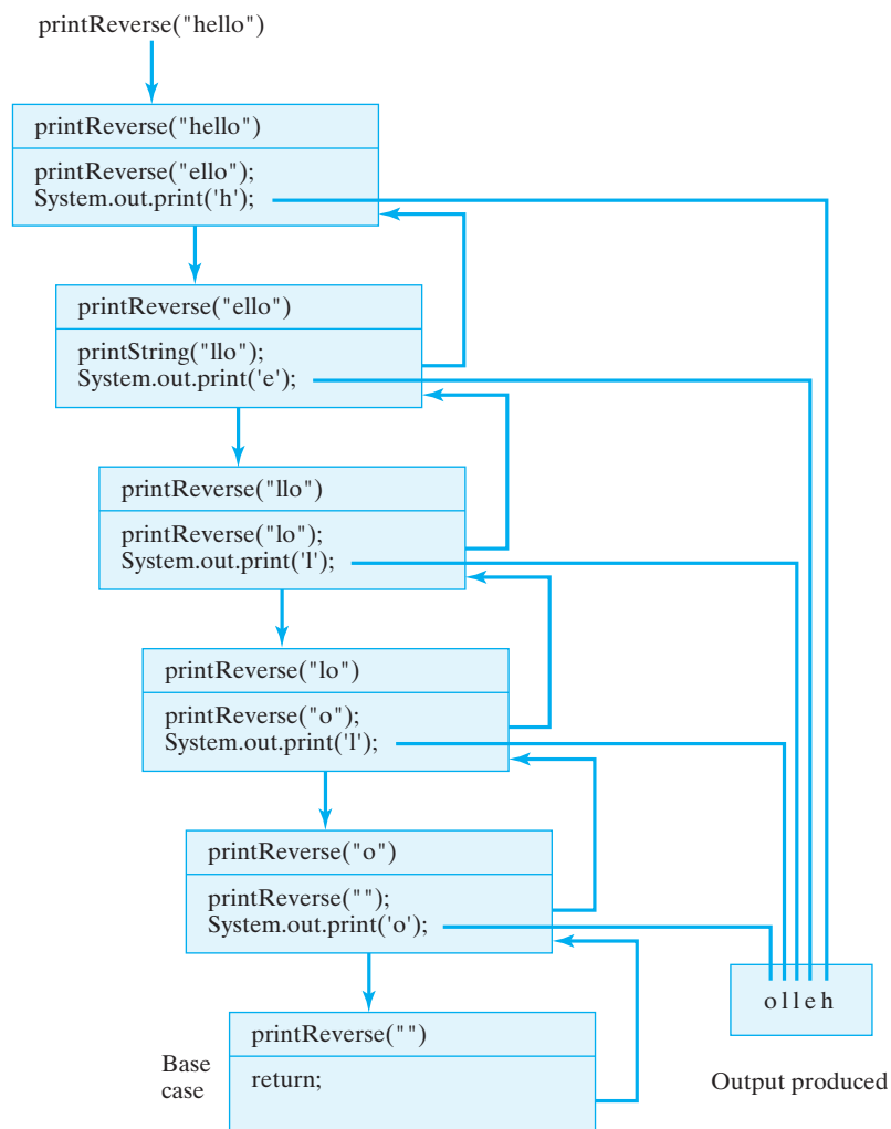
Figure 12.7: A trace of printReverse(s) , which prints its string argument in reverse order.
