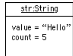
Figure 2.2: A String object stores a sequence of characters and a count giving the number of characters.
