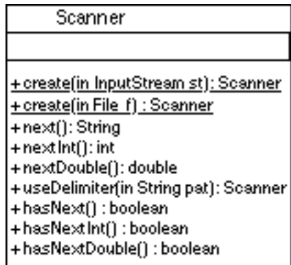
Figure 4.25: A UML class diagram of the Scanner class with an expanded list of public methods
