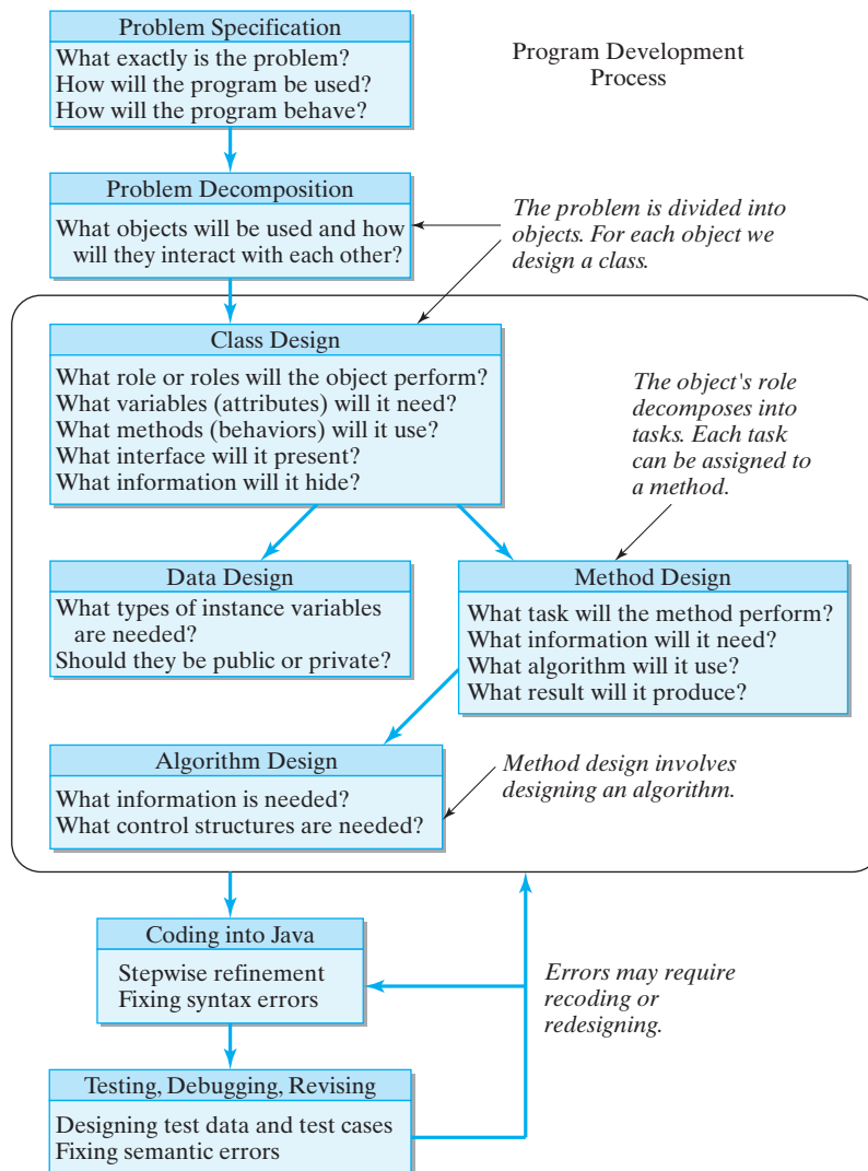
Figure 1.1: An overview of the program development process.
