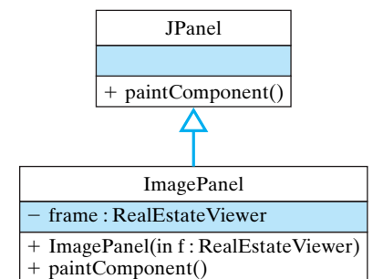
Figure 15.18: An overview of the ImagePanel class.
