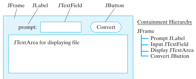
Figure 13.10: A design and layout for the Metric Converter GUI. The containment hierarchy (also called a widget hierarchy ) shows the containment relationships among the components.
