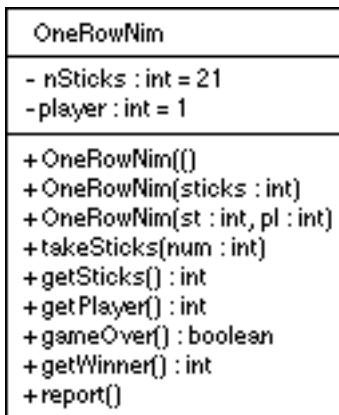
Figure 4.21: A UML diagram of the OneRowNim class.
