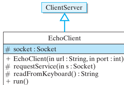
Figure 15.29: Design of the EchoClient class.
