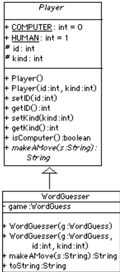
Figure 9.33: The WordGuesser class extends Player.
