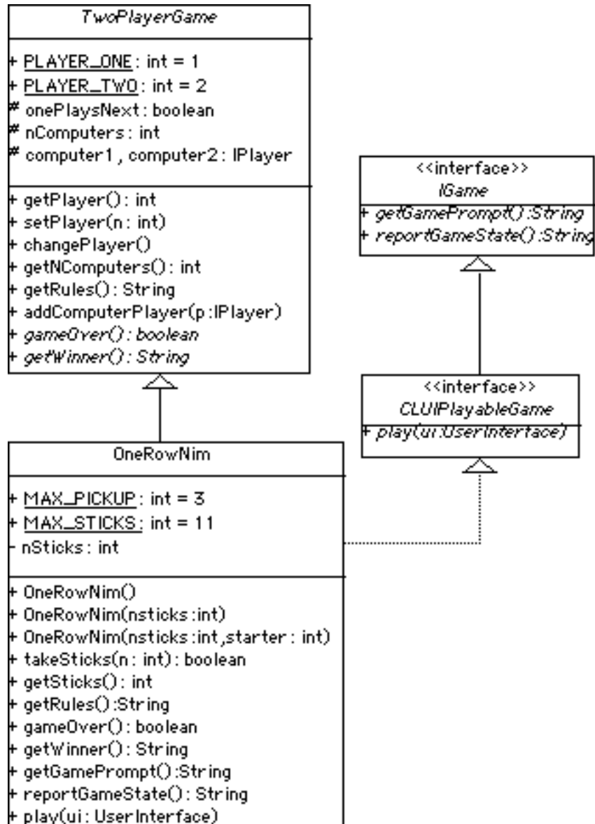
Figure 8.19: TwoPlayerGame is the superclass for OneRowNim and other two player games.
