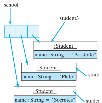
Figure 9.4: Arrays of objects store references to the objects, not the objects themselves.
