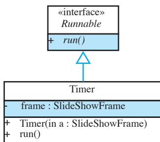
FIGURE 15.11 The Timer class delays the frame thread between each slide.
