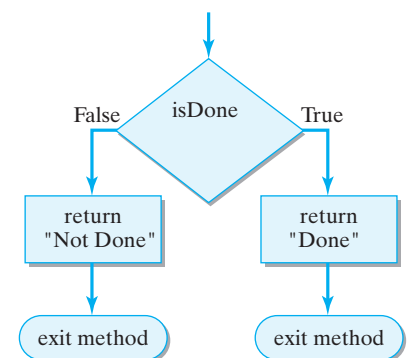
Figure 3.21: Flowchart of the if-else version of the getStatus() method.
