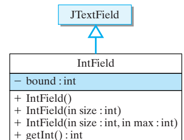
Figure 10.21: The revised IntField class contains a bound on the size of the numbers that should be entered.
