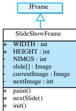
Figure 15.10: The SlideShowFrame downloads and displays the images.
