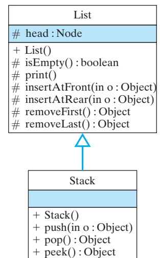
Figure 16.21: As a subclass of List , a Stack inherits all of its public (+) and protected (#) elements. Therefore, push() can be defined in terms of insertAtFront() and pop() can be defined in terms of removeFirst() .
