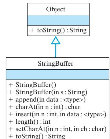
Figure 7.10: The java.lang.StringBuffer class.
