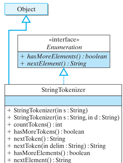
Figure 7.17: The java.util.StringTokenizer class.
