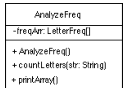
Figure 9.11: UML for AnalyzeFreq.
