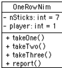
Figure 2.16: A UML class diagram for OneRowNim.
