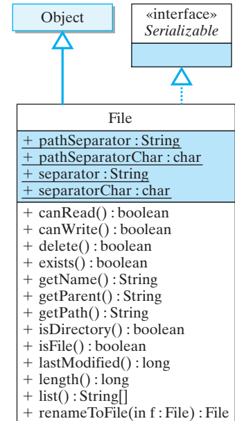
Figure 11.16: The java.io.File class.
