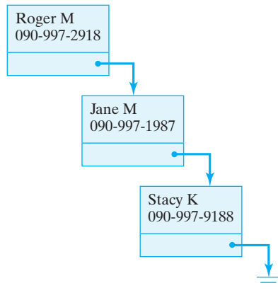
Figure 16.5: The phone list: a linked list of nodes, each of which contains a person's name and phone number.
