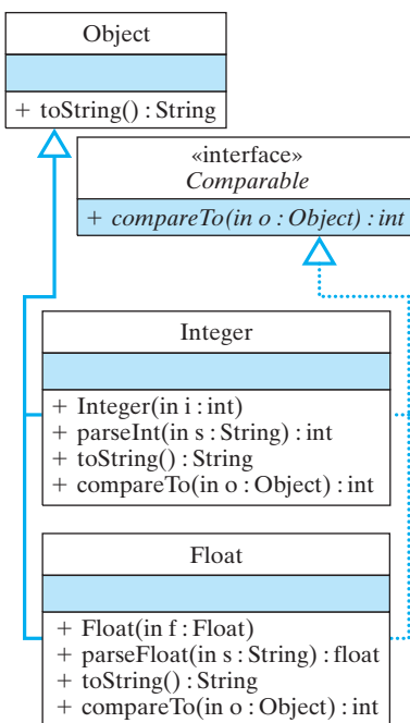
Figure 9.24: Java wrapper classes, such as Integer and Double , implement the Comparable interface.
