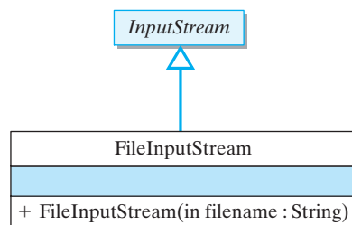
Figure 11.20: The java.io.FileInputStream class.
