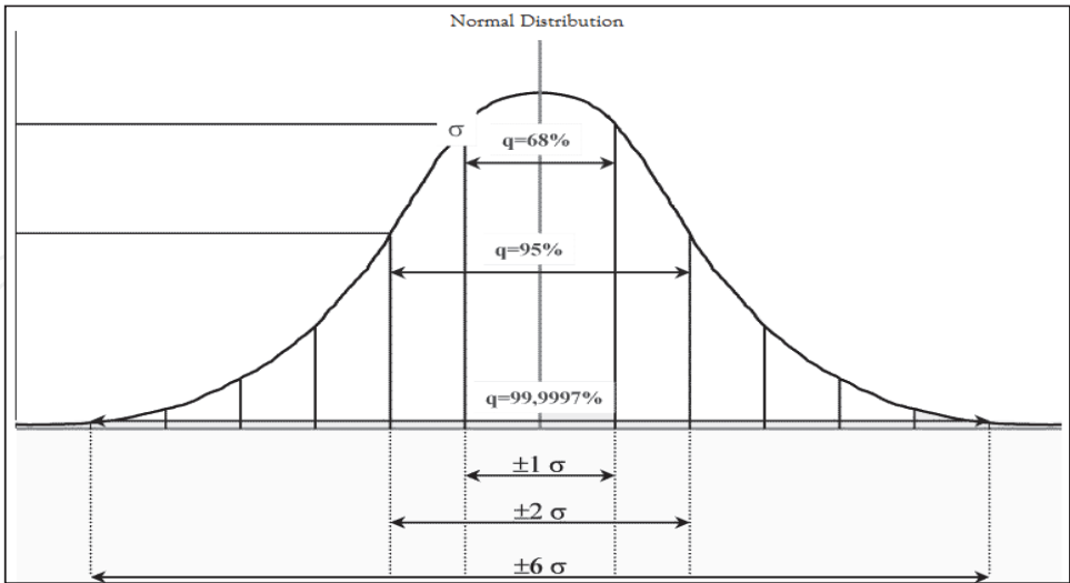
Fig. 3. Normal Distribution
