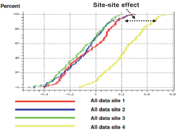
Fig. 8. Temperature Sensor Offset – Replotted by Site.
