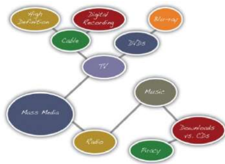
Figure 7.2 Idea Map
