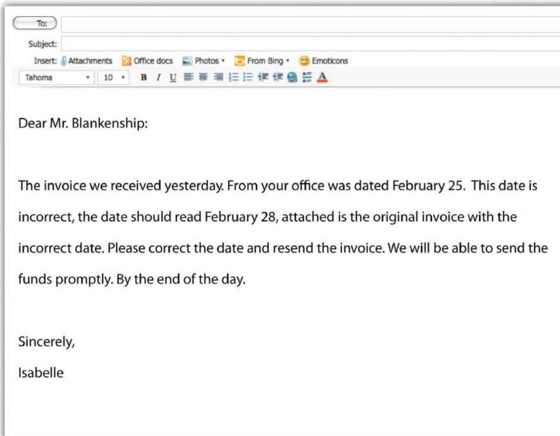
Figure 1.4 Sample e-mail
