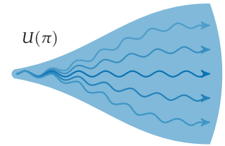
Figure 10.1. The utility associated with a policy from an initial state distribution is computed from the return associated with all possible trajectories under the given policy, weighted according to their likelihood.
