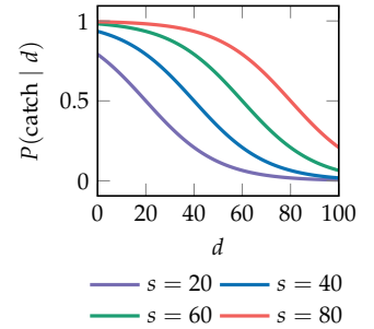
Figure F.13. The catch probability as a function of throw distance d for the four proficiencies in \mathcal{S} .
