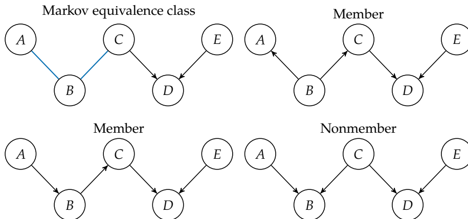
Figure 5.5. A Markov equivalence class and examples of members and a nonmember. The nonmember does not belong to the Markov equivalence class because it introduces an immoral v-structure, A \rightarrow B \leftarrow C , which is not indicated in the partially directed graph.
