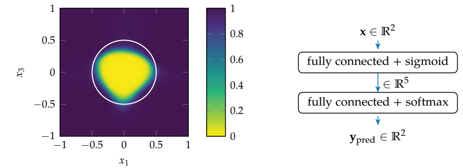
Figure D.4. A simple, two-layer, fully connected network trained to classify whether a given coordinate lies within a circle (shown in white). The nonlinearities allow neural networks to form complicated, nonlinear decision boundaries.
