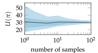
Figure 10.2. The effect of the depth and sample count for Monte Carlo policy evaluation of a uniform random policy on the cart-pole problem (appendix F.3). The variance decreases as the number of samples increases. The blue regions indicate the 5% to 95% and 25% to 75% empirical quantiles of U(\pi) .
