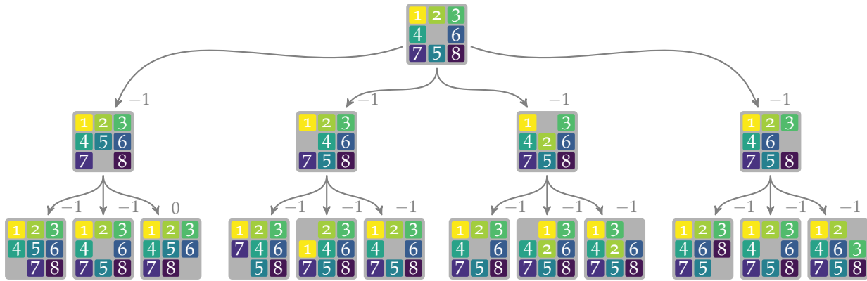
Figure E.3. A search tree arising from running forward search to depth 2 on a sliding tile puzzle. All states reachable in two steps are visited, and some are visited more than once. We find that there is one path to the terminal node. That path has a return of -1 , whereas all other paths have a return of -2 .
