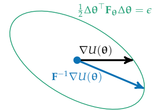
Figure 12.3. The natural policy gradient places a constraint on the approximated Kullback-Leibler divergence. This constraint takes the form of an ellipse. The ellipse may be elongated in certain directions, allowing larger steps if the gradient is rotated.
