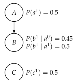
Figure 5.1. A simple Bayesian network to illustrate how the Bayesian score helps us balance model complexity.
