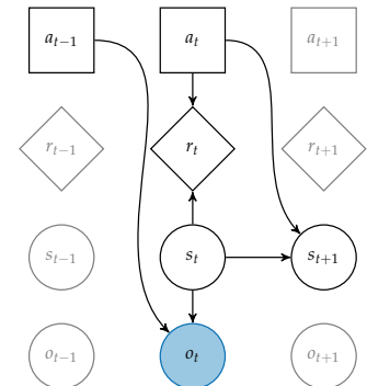
Figure 19.1. A dynamic decision network for the POMDP problem formulation. As with figure 7.1, informational edges into the action nodes are not shown.
