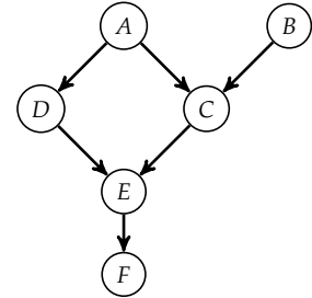
Figure A.6. An example of a graph. Here, \text{Pa}(C) = \{A, B\} . The sequence (A, C, E, F) is a directed path, and (A, C, B) is an undirected path. Node A is a parent of C and D . Node E is a descendant of B . Neighbors of C include A , B , and E .
