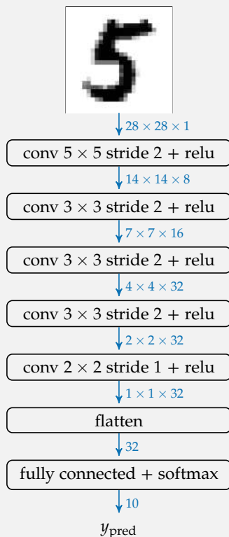
Example D.3. A convolutional neural network for the MNIST data set. Y. LeCun, L. Bottou, Y. Bengio, and P. Haffner, "Gradient-Based Learning Applied to Document Recognition," Proceedings of the IEEE , vol. 86, no. 11, pp. 2278–2324, 1998.
