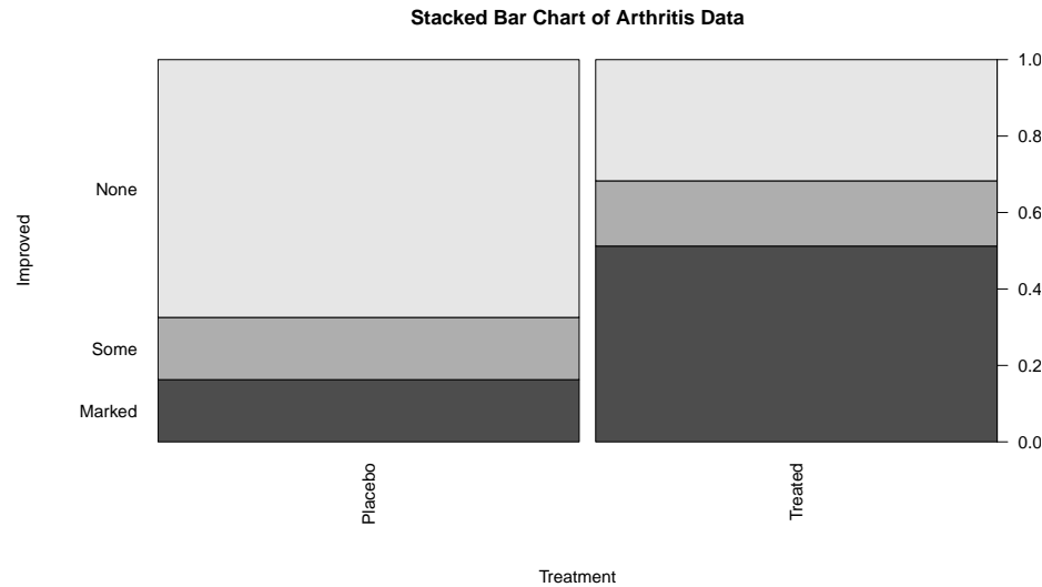
Figure 5.2: Stacked bar chart of Arthritis data. The left bar is for the Placebo group and the right bar is for the Treated group. The width of the bars is based on relative size of each group and the portion of the total height of each shaded area is the proportion of that group in each category. The lightest shading is for “none”, medium shading for “some”, and the darkest shading for “marked”, as labeled on the y-axis.
