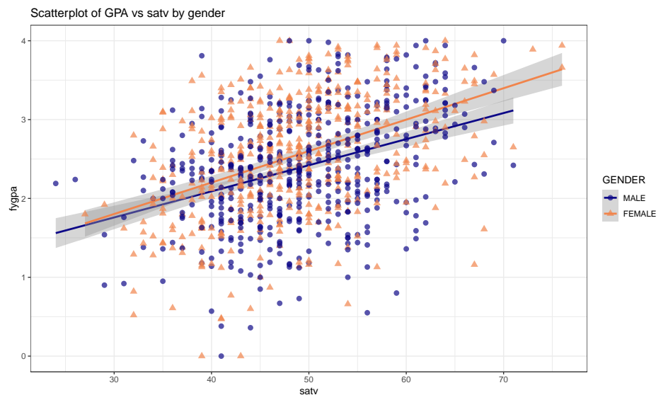
Figure 8.22: Plot of fyghpa vs satv by gender of students.
