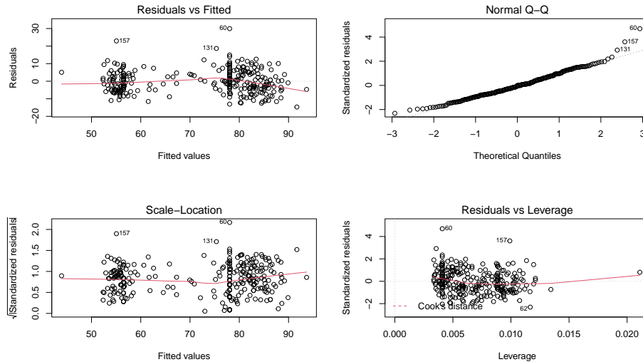
Figure 6.25: Diagnostic plots for Old Faithful waiting time model.
