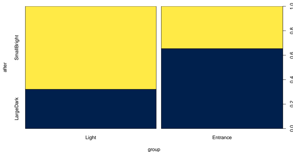
Figure 9.9: Stacked bar chart for Ant Colony results.
