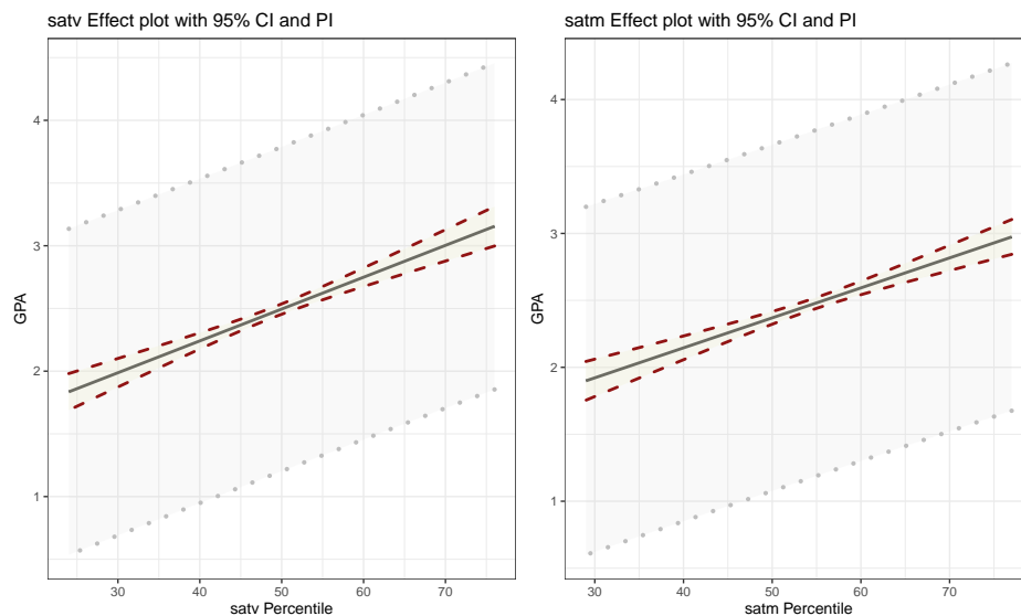
Figure 8.21: Term-plots for the \text{fgpa} \sim \text{satv} + \text{satm} model with 95% confidence intervals (dark, dashed lines) and 95% PIs (light grey, dotted lines).
