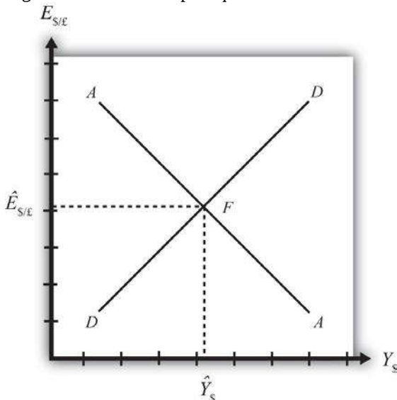
Figure 9.7 AA-DD Superequilibrium
