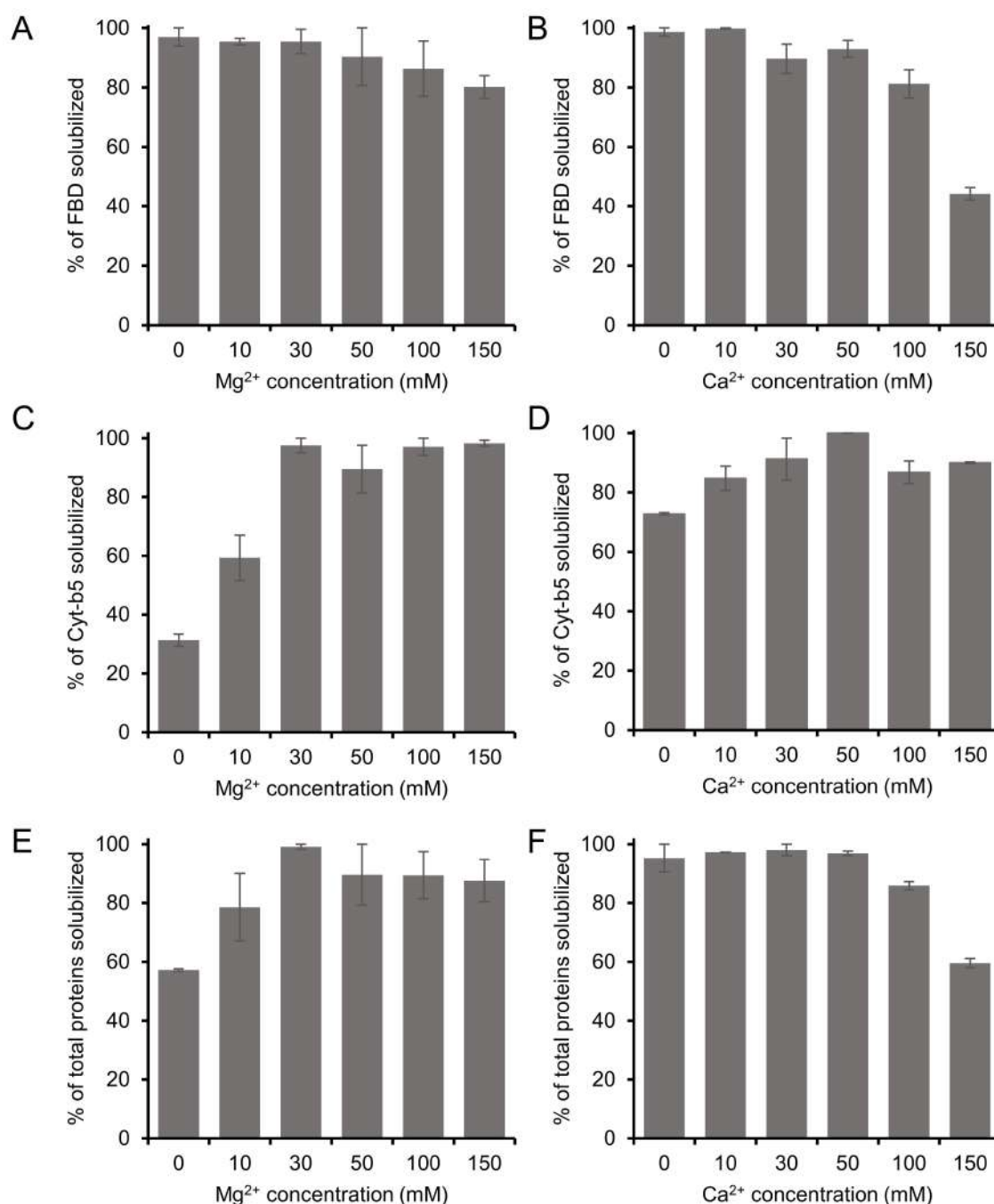
Figure 5. Influence of divalent metal ions ( \text{Mg}^{2+} and \text{Ca}^{2+} ) on the solubilization of E. coli membranes enriched with ( A, B ) FBD, ( C, D ) Cyt-b5 and ( E, F ) total membrane proteins. The
