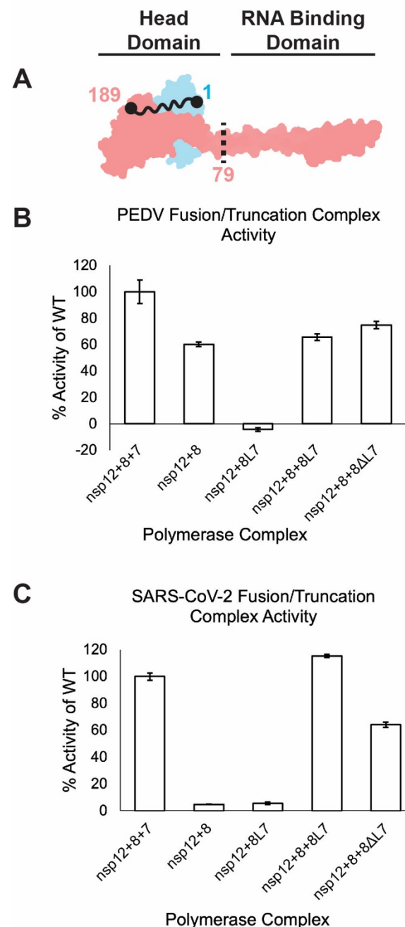
Figure 4: nsp8's N-terminal domain is not required for RNA synthesis. A) Model of nsp7 (blue) and nsp8 (red) heterodimer (PDB ID: 7KRP). The black dots and squiggly line depict the nsp8 and nsp7 termini that are fused in nsp8L7. The dashed black line is the site of truncation of nsp8ΔL7, removing the nsp8 2 N-terminal 79 amino acid RNA binding domain. B) PEDV and C) SARS-CoV-2 polymerase complex activity using the nsp8L7 and nsp8ΔL7 co-factors. Reactions were run in triplicate and percent activity was compared to a wildtype nsp7+nsp8+nsp12 complex. Error bars indicate standard deviation of the triplicates. Each reaction was determined to be significantly different than all other complexes tested ( p < 0.05 ) using an unpaired t-test.
