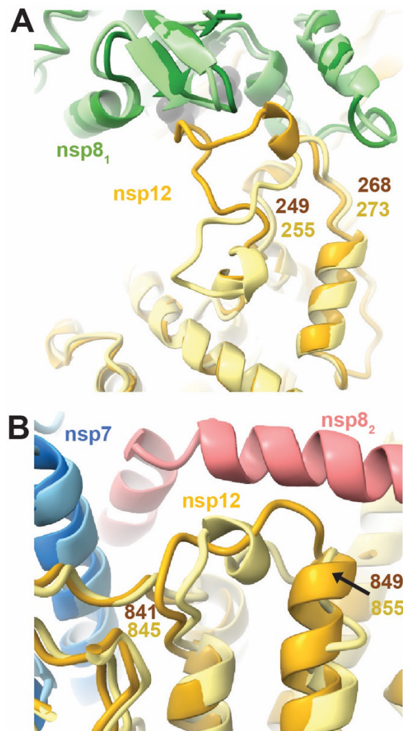
Figure 2: Structural differences between PEDV and SARS-CoV-2 nsp12s. A) PEDV nsp12 loop (residues 249-268) buries extra surface area on nsp8 1 compared to SARS-CoV-2 (PDB: 7KRP). B) PEDV nsp12 841-849 lacks helical definition in the absence of nsp8 2 , while SARS-CoV-2 nsp12 845-855 (PDB: 7KRP) has a short helix when the nsp8 2 N-terminal extension is present. For each panel PEDV and SARS-CoV-2 models are superimposed with PEDV being colored in darker shades. Note that nsp8 2 is not observed in the PEDV structure.
