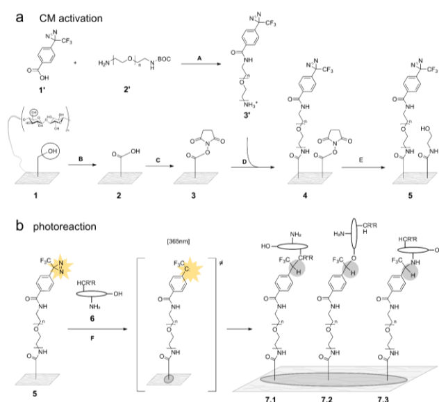
Scheme 1. (a) Construction of a photocrosslinkable cellulose matrix: (top) Functionalization of 4-[3-(trifluoromethyl)-3H-diazirin-3-yl]benzoic acid (TDBA) (1') with an amine-reactive PEG-spacer of variable length using Boc-NH-PEGn-CH 2 CH 2 NH 2 (2') to create a primary amine-containing trifluoromethylphenyldiazirine (TPD) (3'). (bottom) Stepwise activation of cellulose membranes (1) by TEMPO-mediated oxidation to get oxidized cellulose (2) and activation with NHS and 1-Ethyl-3-(3-dimethylaminopropyl)carbodiimide (EDC) to obtain NHS-activated cellulose (NAC) (3). Immobilization of the photocrosslinker (3') on the activated cellulose (3) to form the TPD-functionalized cellulose (TFC) (4). Blocking of unreacted NHS-groups to obtain a blocked TFC membrane (5). (b) reaction principle of undirected photocrosslinking: spotting of constructed affinity matrix (5) with a compound solution of interest, here represented by a fictional compound (6), evaporation of the solvent, formation of reactive carbene induced by irradiation with UV-light at 365 nm, formation of different reaction products (7.1, 7.2, 7.3) of undirected photocrosslinking reaction between photoactivated 5 and dried compound of interest (6). Reaction conditions: (A) 1 eq. TDBA, 1.25 eq. Boc-N-amido-PEG-amine, 0.35 eq. 4-Dimethylaminopyridine (DMAP), 30 min, THF; 1.75 eq. EDC, 18 h, RT, dark; (B) NaOH (w(NaOH) = 10%), 18 h, H 2 O, RT; 0.39 mmol TEMPO, 14.1 mmol NaBr, 17.0 mmol NaOCl, 1 h, H 2 O, pH 10; (C) 30 mmol NHS, 0.4 mol/l EDC, sodium acetate, 1.5 h, H 2 O, pH 5; (D) 10 mM amine-PEG TPD, 21 h, THF, RT; (E) 1-3 M ethanolamine (EA), 1-2 h, H 2 O; (F) 10 mM compound solution, drying, irradiation at 365 nm.
