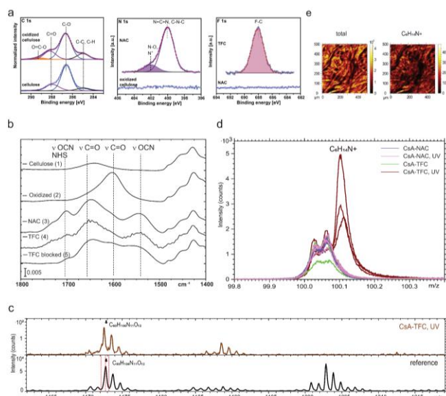
Figure 2. XPS, ATR-FTIR and ToF-SIMS spectra of stepwise cellulose functionalization. (a) C 1s XPS spectra for unmodified and oxidized cellulose (left), N 1s photoelectrons for oxidized and NHS-activated cellulose (NAC, center) and F 1s photoelectrons of NHS-activated and TPD-functionalized cellulose (TFC, right). (b) Selected region of ATR-FTIR spectra of unmodified and functionalized cellulose. (c) ToF-SIMS spectra of a CsA reference sample (drop-cast, bottom) and CsA-spotted TFC after UV irradiation (top) over a mass range of m/z 1160-1220. (d) ToF-SIMS spectrum in the mass range of the amino acid fingerprinting signal of N-methylated Leu ( C_6H_{14}N^+ , m/z 100) across different samples: CsA spotted NAC (NHS-activated cellulose, purple), CsA-spotted UV-treated NAC (pink), CsA spotted TFC (green) and CsA spotted TFC and treated with UV (brown). Spectra were acquired at three different lateral positions across the corresponding sample. (e) ToF-SIMS chemical mapping showing the lateral distribution of different CsA-fragment signals across CsA spotted TFC irradiated with UV.
