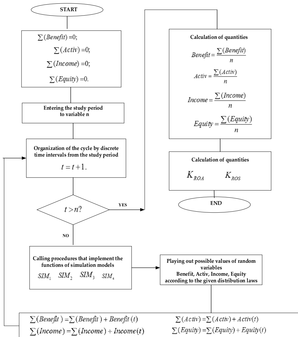
Figure 2. The algorithm of functioning of factor models for financial analysis DP_2 , DP_3 .
