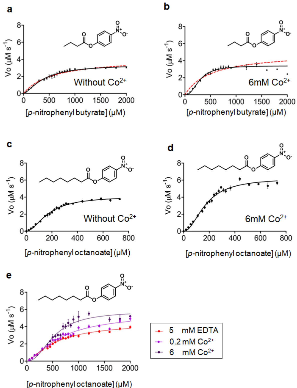
Figure 5. Hydrolysis of substrates p -nitrophenyl butyrate and p -nitrophenyl octanoate. Kinetic activity of Ade1 in presence of different substrates. p -nitrophenyl butyrate in (a) absence and (b) presence of 6 mM \text{Co}^{2+} . p -nitrophenyl octanoate in (c)
