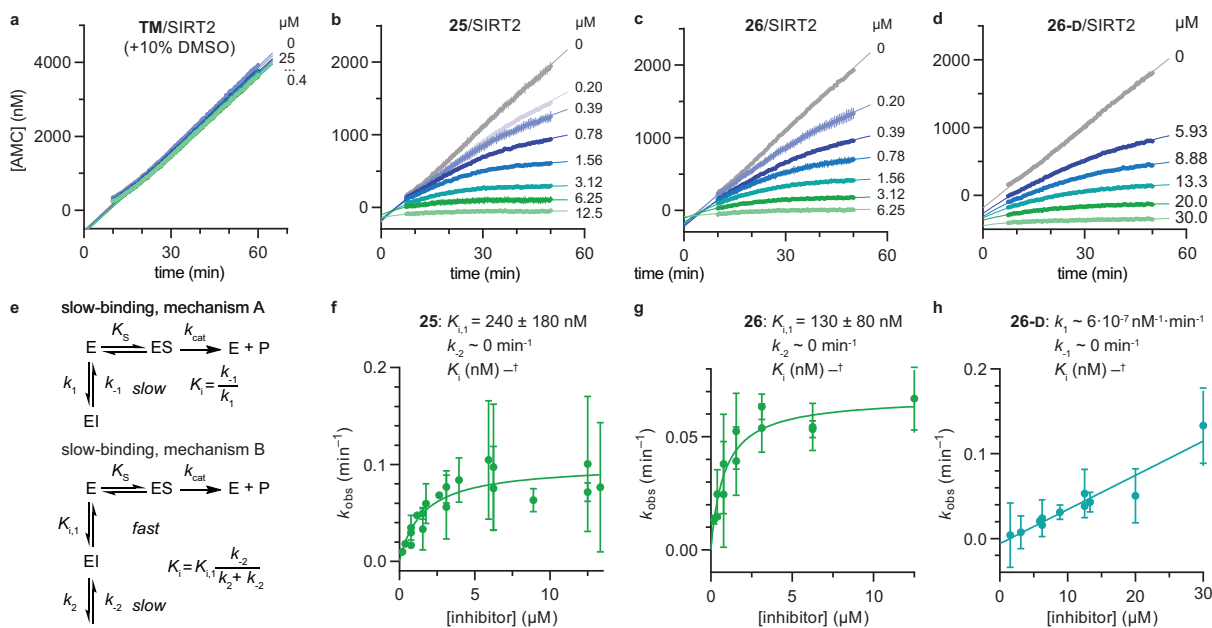
Fig. 3. Kinetics of SIRT2 inhibition by compounds 25, 26, and 26-D. Sample rate experiment curves for compounds (a) TM, (b) 25, (c) 26, and (d) 26-D, with concentration of inhibitor for each experiment indicated on the right of the curve. (e) Common mechanisms of slow-binding inhibitor kinetics, with associated equilibrium and rate constants. Dependence of the first-order rate constant to reach steady state ( k_{obs} ) on inhibitor concentration for compounds (f) 25 and (g) 26, following mechanism B, and (h) 26-D, which follows mechanism A. Continuous assays were performed with SIRT2 (20 nM), ETDKmyr (20 μM) as substrate, trypsin (20 ng/μL), and at designated inhibitor concentrations. See Table S3 for additional details and complete data fitting.
