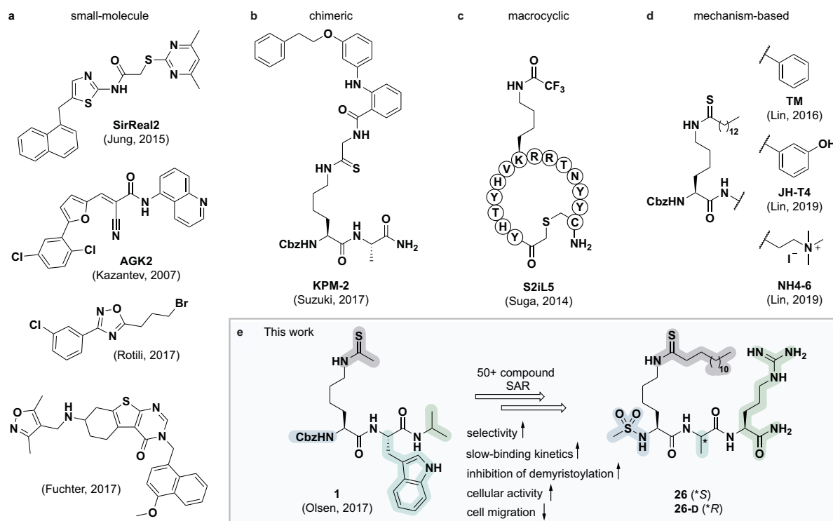
Fig. 1. Representative SIRT2 inhibitors. (a) Heterocyclic small molecule inhibitors. 30,35,46,47 (b) Chimeric lysine mimic KPM-2. 37 (c) Peptide macrocycle S2iL5. 34 (d) Mechanism-based inhibitors. 24,32,40 (e) Summary of this study.
