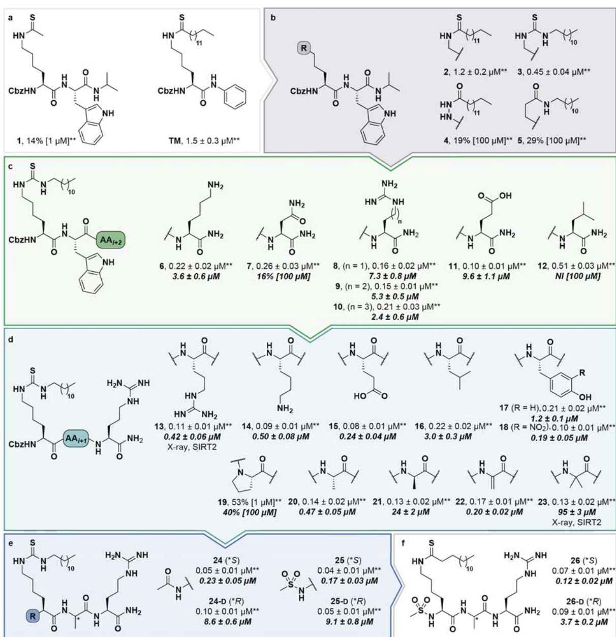
Scheme 1. Structure–activity relationship of SIRT2 inhibitors. Potencies for inhibition of the deacetylase activity of recombinant SIRT2 (100 nM) against QPKKac (shown with asterisks**) or ETDKmyr (shown in bold/italics) as substrate (50 \mu\text{M} ) are given as mean IC 50 values \pm standard deviation (SD) or %-inhibition. (a) Lead compounds. (b) Amide isosteres. (c) Optimization of position i +2. (d) Optimization of position i +1. (e) Optimization of N -terminal group. (f) Final inhibitor series. Data are based on two individual experiments performed in duplicate. See the Supplementary Information (Scheme S1, Fig. S1–S3, and Table S2) for dose–response curves and selectivity profiling of additional inhibitors (S17–S23) against SIRT1–3. *A single asterisk denotes a stereogenic center.
