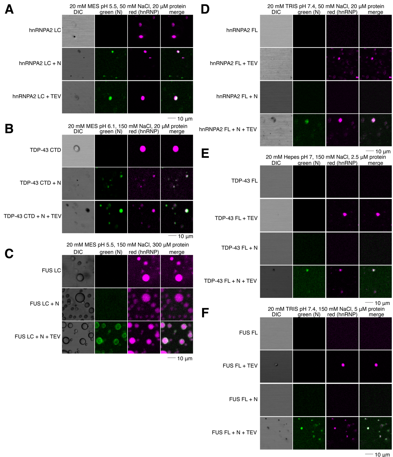
Figure 5: SARS-CoV-2 N partitions into liquid phases of hnRNPs. A) N partitions into hnRNP2 LC droplets even with the MBP tag attached. B) N partitions into TDP-43 CTD droplets even with the MBP tag attached. C) N partitions into FUS LC droplets only after cleavage of the MBP tag. D-F) N partitions into hnRNP2 FL (D), TDP-43 FL (E), FUS FL (F) droplets.
