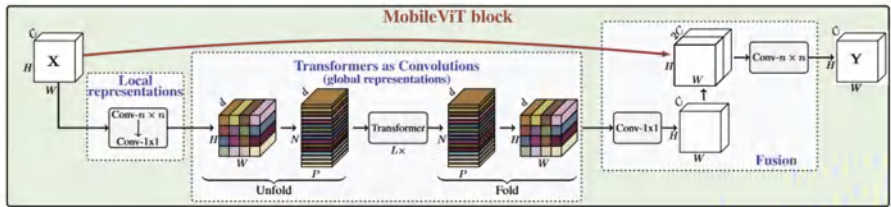
Figure 5.4 MobileViT block [37].
