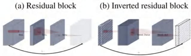
Figure 5.3 MobileNetV2 block
