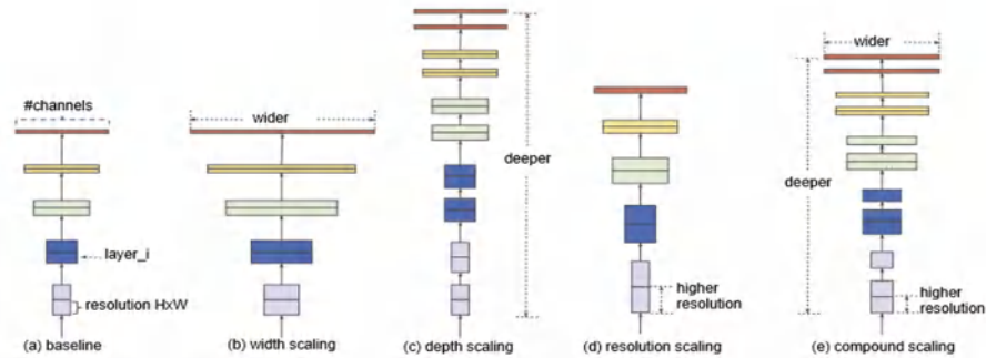
Figure 5.6 EfficientNet Scaling [12]
