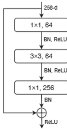
Figure 5.1 ResNet architecture [11]
