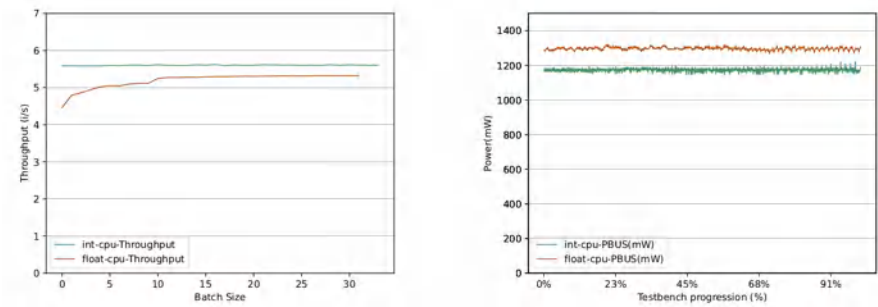
Figure 4.3 MP1 Performance and Power Measurements
