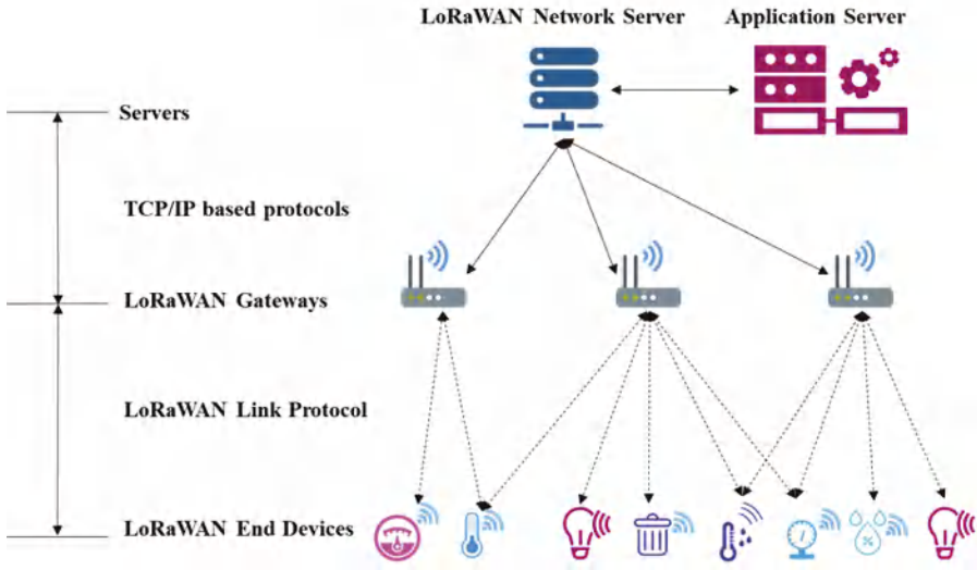
Figure 1.6 LoRaWAN Network Architecture
