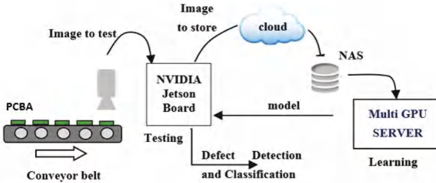
Figure 7.4 AOI Solution Consisting of an Edge Board for Testing and a GPU Server for Learning.
