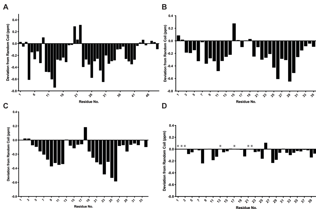
Figure 2 | Secondary H_\alpha shifts of synthetic VBPs. (A) C2; (B) VBP-10; (C) VhTI; and (D) VBP-6. Observed significant negative stretches are indicative of helical regions, with the positive or close to zero values in the center of these negative stretches being consistent with the loop region of the hairpin.
