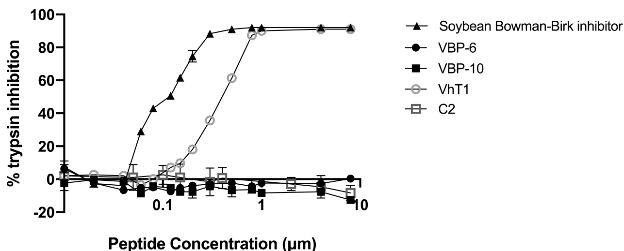
Figure 7 | Inhibition of bovine trypsin by VBPs. Trypsin activity was determined in the presence of C2, VhTI, VBP-6 and VBP-10 at a range of concentrations from 0.01 to 8 \mu M. Soybean Bowman-Birk inhibitor was used as a positive control. The standard error of the mean is shown for each triplicate data point.
