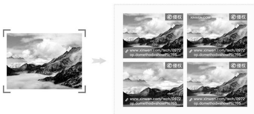
Fig. 1.14 Image search
