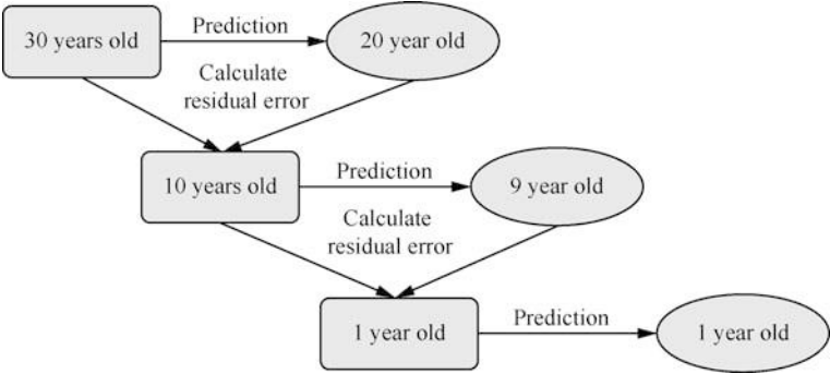
Fig. 2.43 GBDT algorithm
