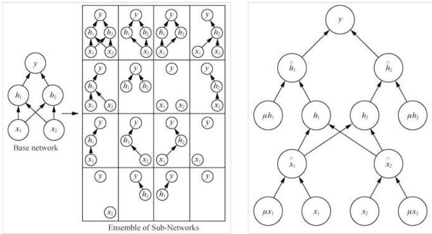
Fig. 3.16 Dropout
