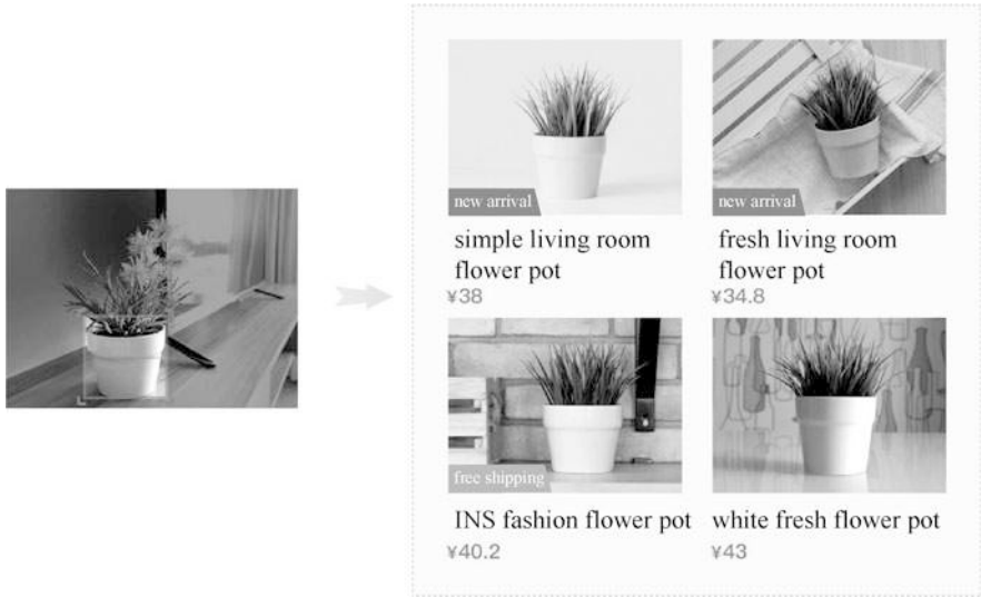
Fig. 8.15 Commodity search
