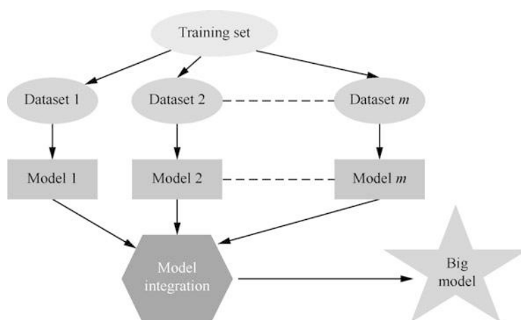
Fig. 2.41 Ensemble learning
