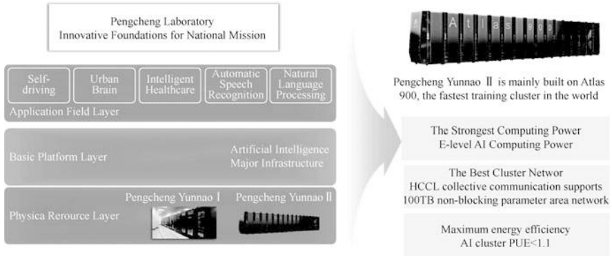
Fig. 6.43 Pengcheng laboratory
