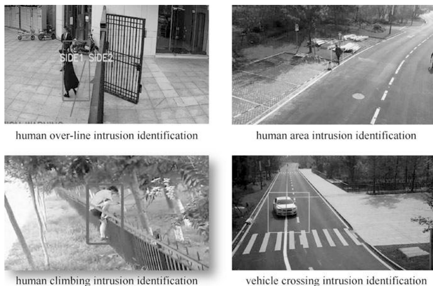
Fig. 8.30 Intrusion identification
