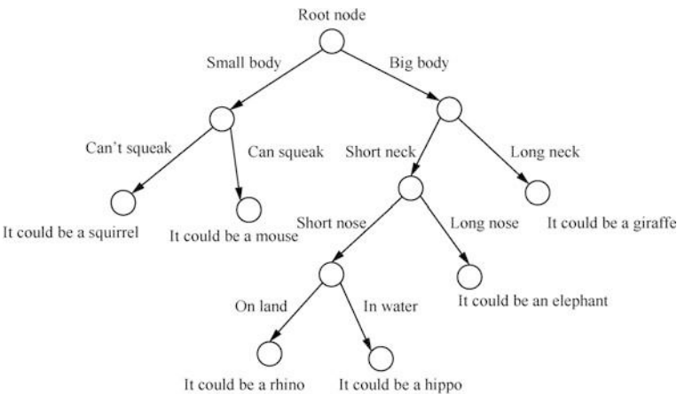
Fig. 2.35 An example of decision tree
