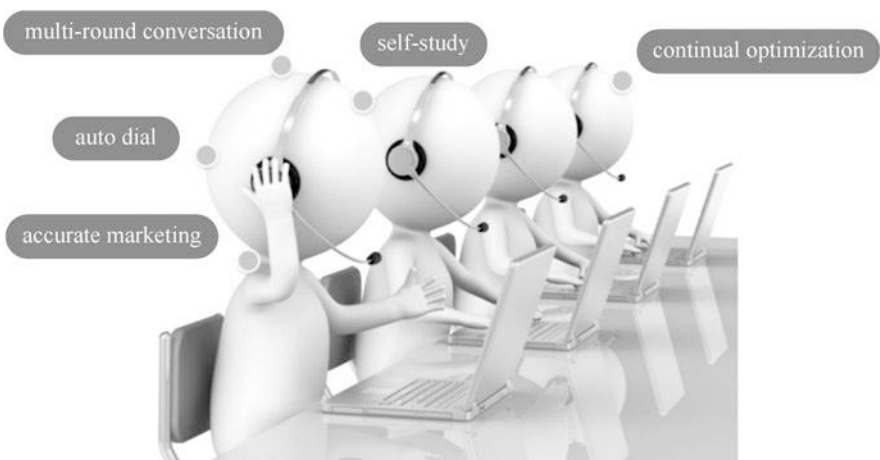
Fig. 8.9 Conversational bot
