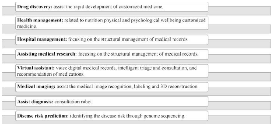
Fig. 1.21 Smart healthcare
