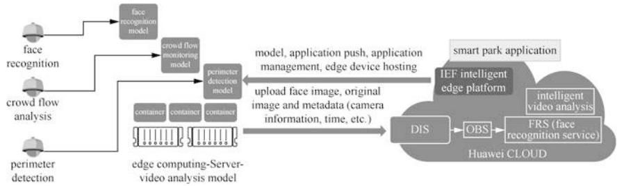
Fig. 8.27 Smart park
