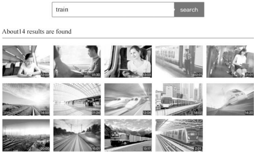
Fig. 8.12 Video search
