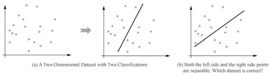
Fig. 2.37 Performance of linear classifier
