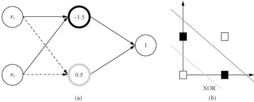
Fig. 3.7 Multilayer perceptron solving the XOR problem
