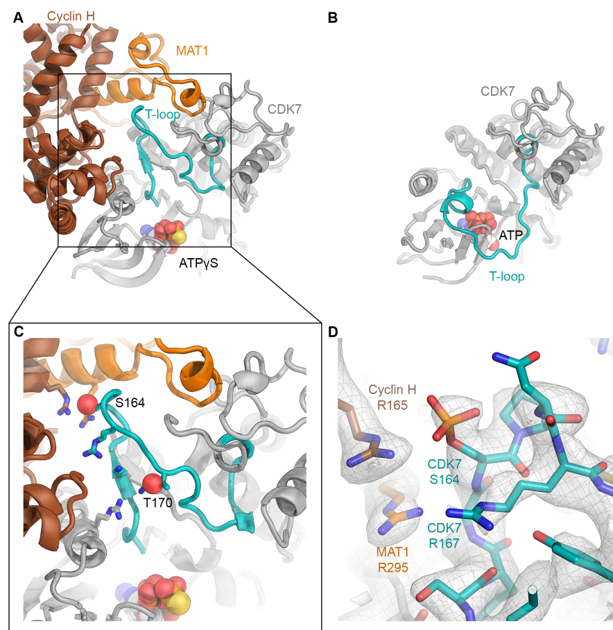
Figure 3. Extended T-loop of CDK7. (A) The T-loop in the CAK-ATPyS complex is extended and points towards MAT1 and cyclin H. (B) In the crystal structure of free, inactive CDK7, the T-loop is folded across the active site (PDB ID 1UA2; shown in the same orientation as CAK in panel A) (Lolli et al., 2004). (C) Positively charged residues near the CDK7 phosphorylation sites (S164, T170; O \gamma shown as red spheres) are shown as sticks. (D) Structure of the CAK near S164; cryo-EM density shown in grey (combined surface and mesh) suggests that S164 is partially phosphorylated in our preparation of CAK. Positively charged residues surrounding the phosphate group are labeled.
