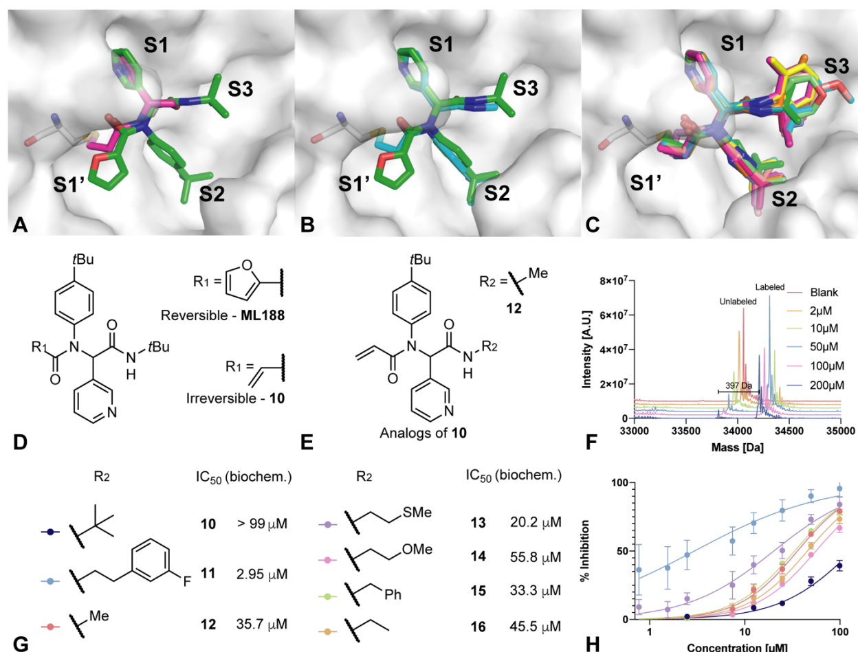
Figure 5. Computational prediction and experimental validation of an irreversible SARS-CoV-2 M pro inhibitor. A. The covalentizer prediction of 10 (magenta) overlaid on the non-covalent compound it is based on (ML188 45 ; green; PDB:3V3M). The protocol suggested to substitute the furanyl moiety of ML188 with an acrylamide to bind the catalytic cysteine. The RMSD between the covalent fragment and the original reversible inhibitor is 0.65 Å. B. The crystal structure of one of the covalent analogs of 10 (PDB: 5RH5; cyan) overlaid on ML188 (green). C. Overlay of all the 11 crystal structures of compound 10 analogs, all exhibiting the same predicted binding mode. PDBs: 5RGT, 5RH5, 5RH6, 5RH7, 5RH9, 5RL0, 5RL1, 5RL2, 5RL3, 5RL4, 5RL5. For individual structures see Supp. Fig. 5. D. The chemical structures of ML188 and 10 . E. Chemical structure of Ugi compounds exploring the S3 pocket, with the R group that is shown in the crystal structure in (B). F. Deconvoluted mass spectra obtained by intact protein LC/MS of recombinant SARS-CoV-2 M pro 2 μM incubated with 2 μM - 200 μM 10 for 1.5 h at room temperature. G. Further analogs of 10 with their associated biochemical potencies. H. The dose response curves for the seven compounds shown in G.
