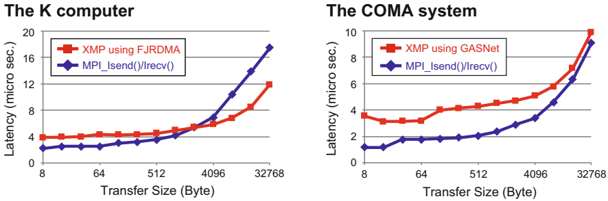
Fig. 20 Performance results for ping-pong benchmark [5]
