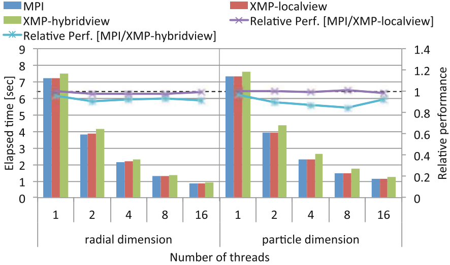
Fig. 20 Elapsed time of the decomposition on radial and particle dimension from 1 to 16 threads
