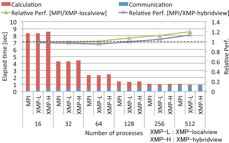
Fig. 17 Elapsed time of the decomposition on radial dimension from 16 to 512 processes in strong scaling
