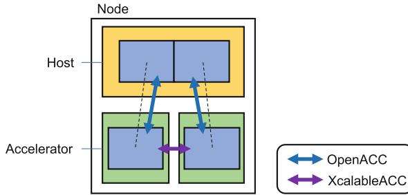
Fig. 3 Concept of OpenACC extension
