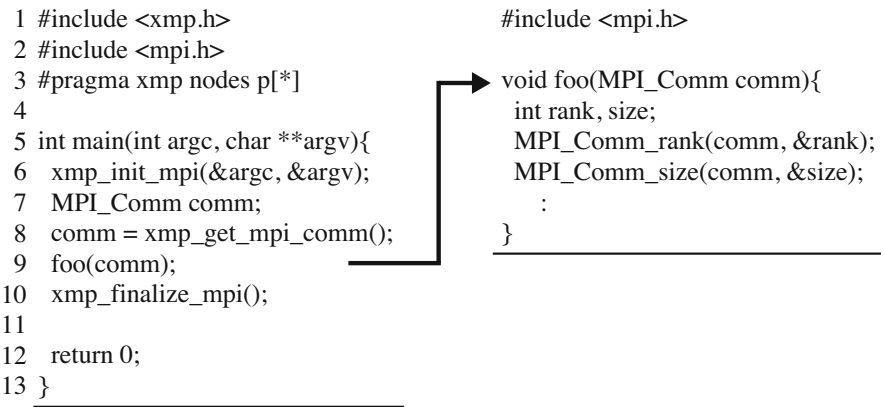
Fig. 2 Example of calling MPI program (mpi.c) from XMP program (xmp.c) [19]
