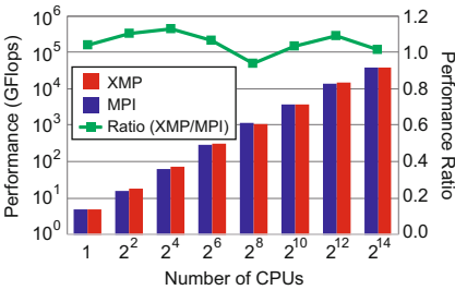
Fig. 16 Performance results for FFT [5]
