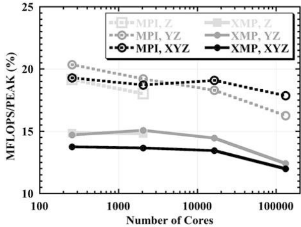
Fig. 3 MFLOPS/PEAK measured by the hardware monitor installed on the K computer with SIMD optimization by simd=2 compiler option. Solid and dash lines indicate performances of XMP and MPI codes, respectively. Colors of light gray, gray, and black indicate only Z domain decomposition, both Y and Z domain decomposition, and all of X, Y, and Z domain decomposition methods, respectively
