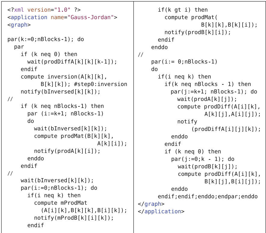
Fig. 5 An example of an application written in YvetteML
