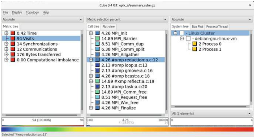
Fig. 5 Profile by Scalasca ( https://omni-compiler.org )
