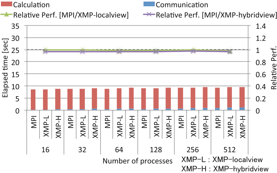
Fig. 14 Elapsed time of the decomposition on particle dimension from 16 to 512 processes in weak scaling
