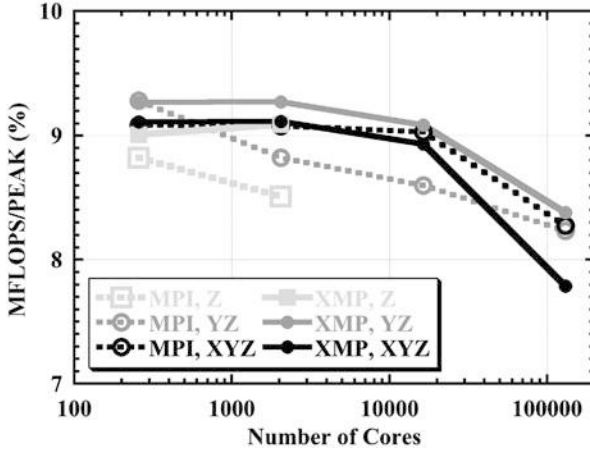
Fig. 2 MFLOPS/PEAK measured by the hardware monitor installed on the K computer. Solid and dash lines indicate performances of XMP and MPI codes, respectively. Colors of light gray, gray, and black indicate only Z domain decomposition, both Y and Z domain decomposition, and all of X, Y, and Z domain decomposition methods, respectively
