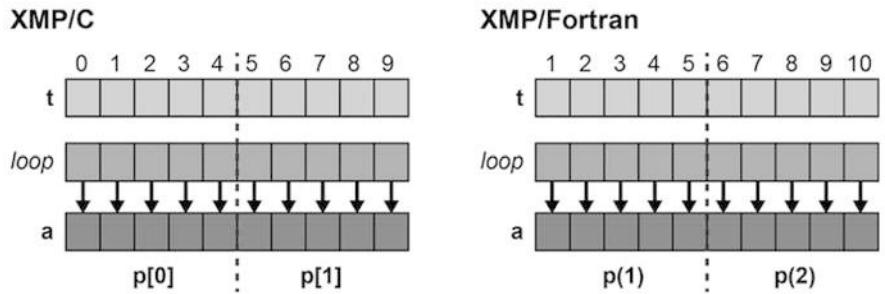
Fig. 22 Example of loop construct (1)
