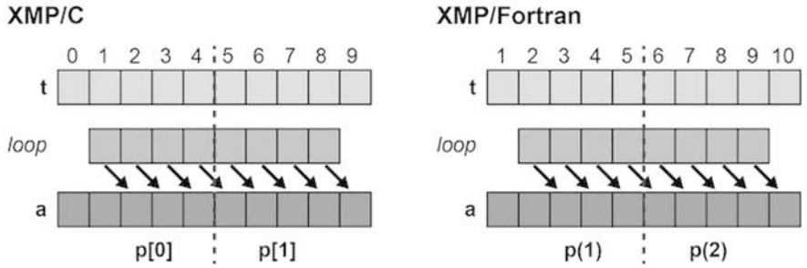
Fig. 24 Example of loop construct (3)
