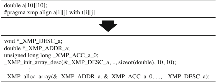
Fig. 2 Code translation of align directive
