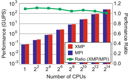
Fig. 18 Performance results for RandomAccess [5]
