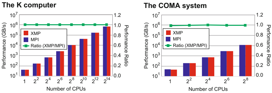
Fig. 9 Performance results for STREAM [5]
