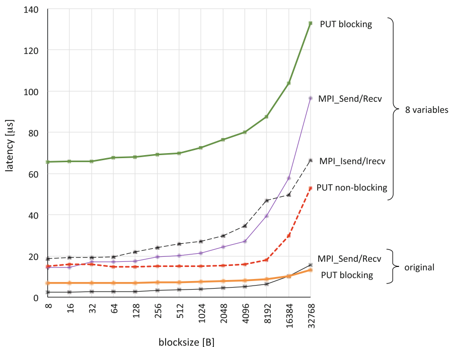
Fig. 7 Eight-variable ping-pong latency on PRIMEHPC FX100
