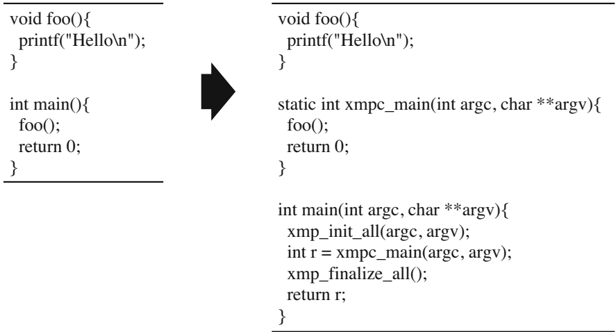
Fig. 1 Example of translation in Omni compiler [19]
