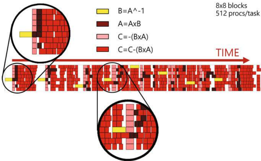
Fig. 9 Execution timeline of the BGG workflow application with 8 \times 8 blocks
