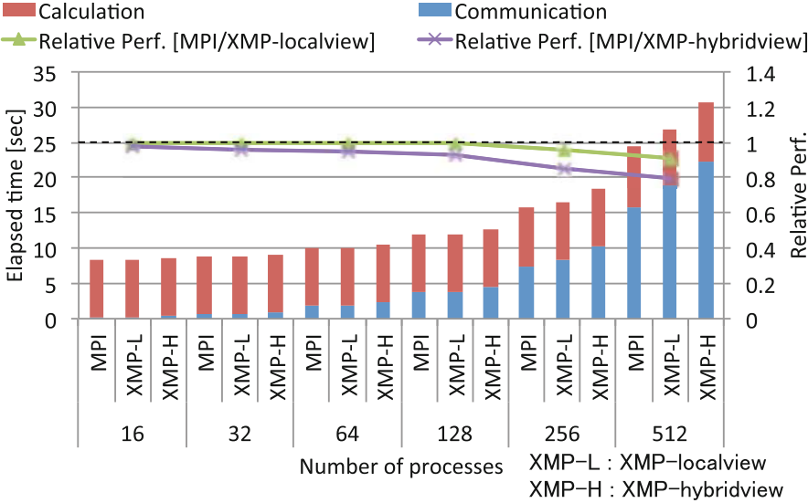
Fig. 13 Elapsed time of the decomposition on radial dimension from 16 to 512 processes in weak scaling
