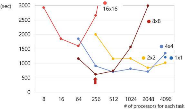
Fig. 8 Execution time of the BGJ workflow applications
