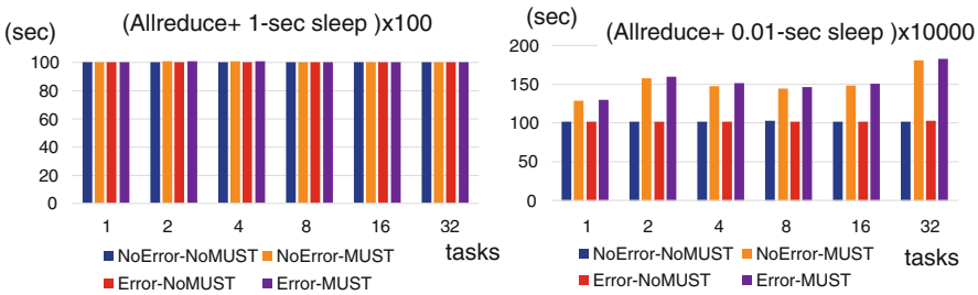
Fig. 22 Execution time when a workflow includes 1, 2, \dots 32 tasks executing MPI_Allreduce repeatedly every 1-s (left) and every 0.01-s
