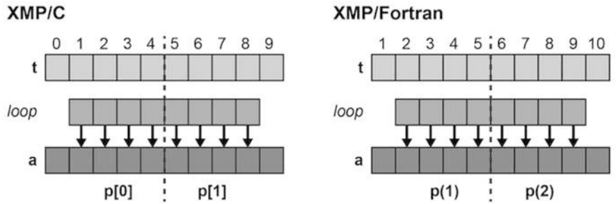
Fig. 23 Example of loop construct (2)
