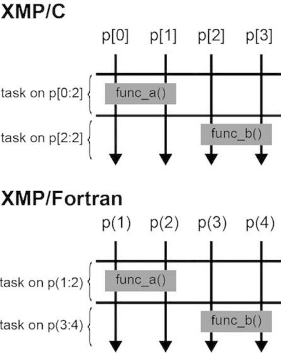
Fig. 20 Example of task construct (2)
