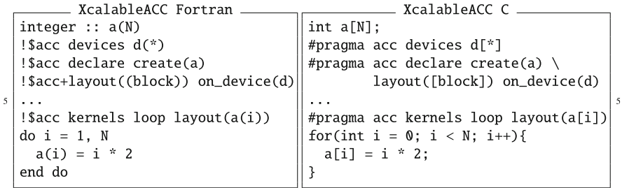
Fig. 10 Xacc Code example with layout clause
