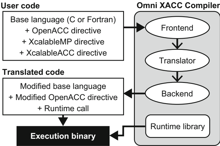
Fig. 13 Compile flow of Omni XscalableACC compiler
