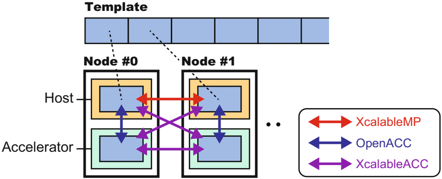
Fig. 2 Concept of XMP extensions
