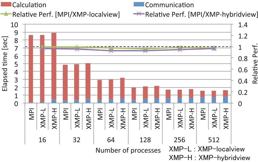
Fig. 18 Elapsed time of the decomposition on particle dimension from 16 to 512 processes in strong scaling
