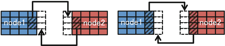
Fig. 21 Updating of the sleeve area with MPI and XMP-localview (left), and XMP-hybridview (right) in GTC-P. The hatching areas are communicated to nearby node
