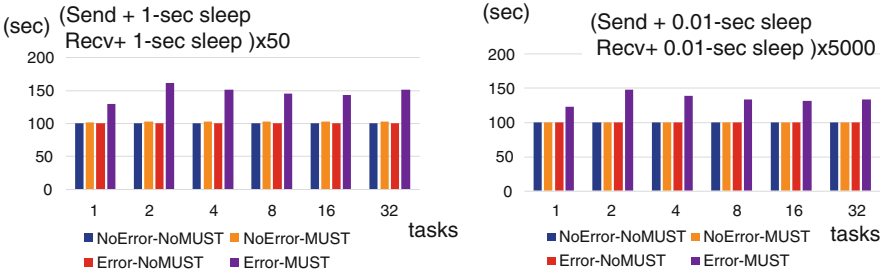
Fig. 23 Execution time when a workflow includes 1, 2, \dots 32 tasks executing MPI_Send/Recv repeatedly every 1-s (left) and every 0.01-s
