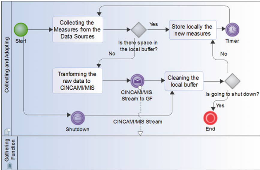
Fig. 9 Details on the collecting activity for the collecting and adapting process using BPMN notation
