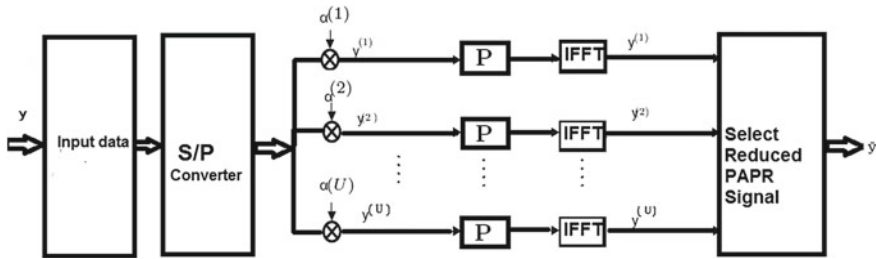
Fig. 9 Proposed SLM technique
