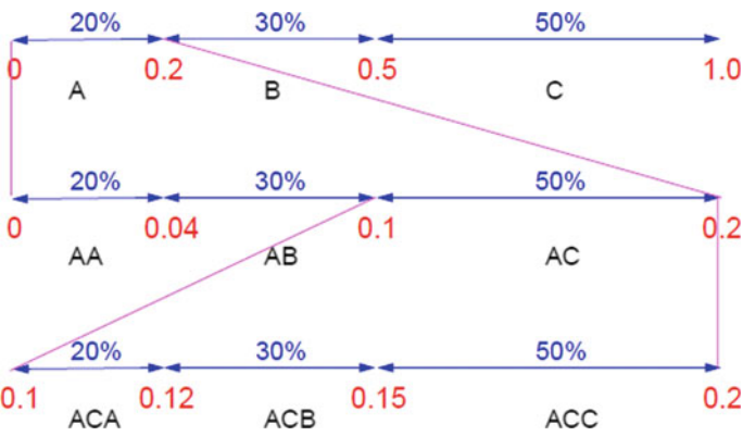
Fig. 4 Code generation for arithmetic coding
