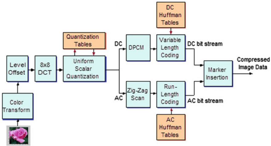
Fig. 6 JPEG algorithm encoding
