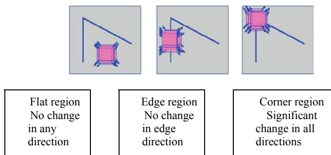
Fig. 2 Harris corner detection
