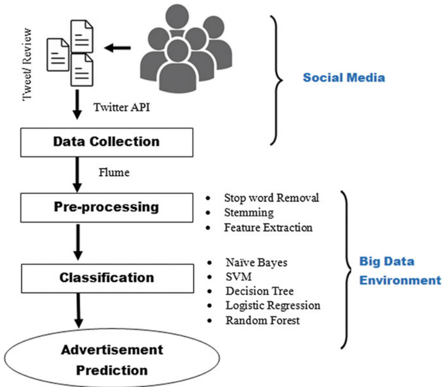
Fig. 4 Advertisement prediction framework
