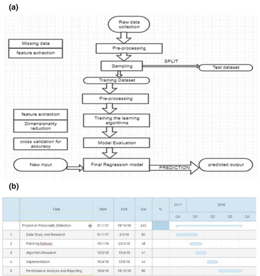
Fig. 4 a Flowchart of regression analysis. b Gantt chart of activity
