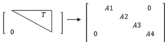
Fig. 2 Modified T matrix as a four block T^{\wedge} [21]
