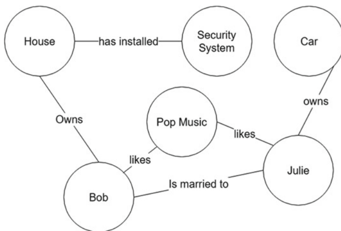
Fig. 14 Graph data
