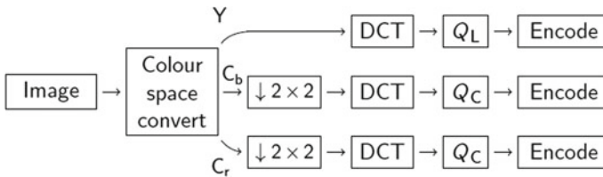
Fig. 5 Functional steps of JPEG image compression
