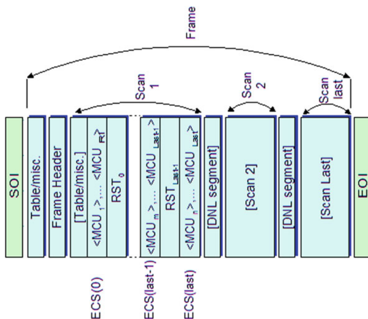
Fig. 9 Simple compressed image data format
