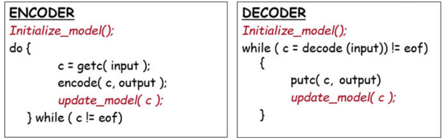
Fig. 2 Huffman encoding procedure
