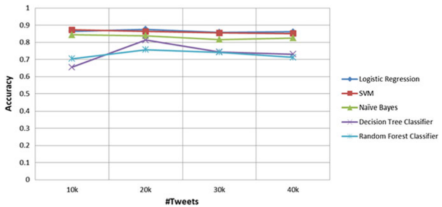
Fig. 9 Accuracy comparison
