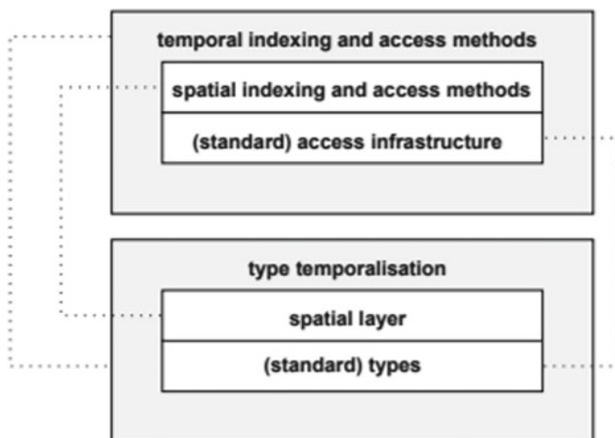
Fig. 10 The storage manager in a spatio-temporal DBMS
