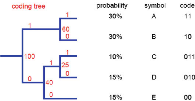
Fig. 2 Huffman encoding procedure
