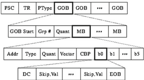
Fig. 16 Encoding sequence
