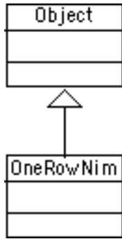
Figure 2.16: A UML class diagram for OneRowNim.
