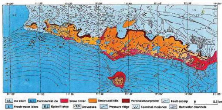
Figure 3. Geomorphological map of Schirmacher oasis.
