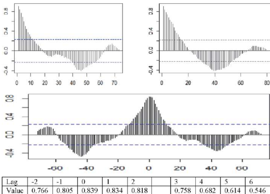
Figure 5. Cycle C1 temperature and CO 2 autocorrelations (left to right, above) and cross correlation (below) indicating some periodicity within the cycle C1 itself.
