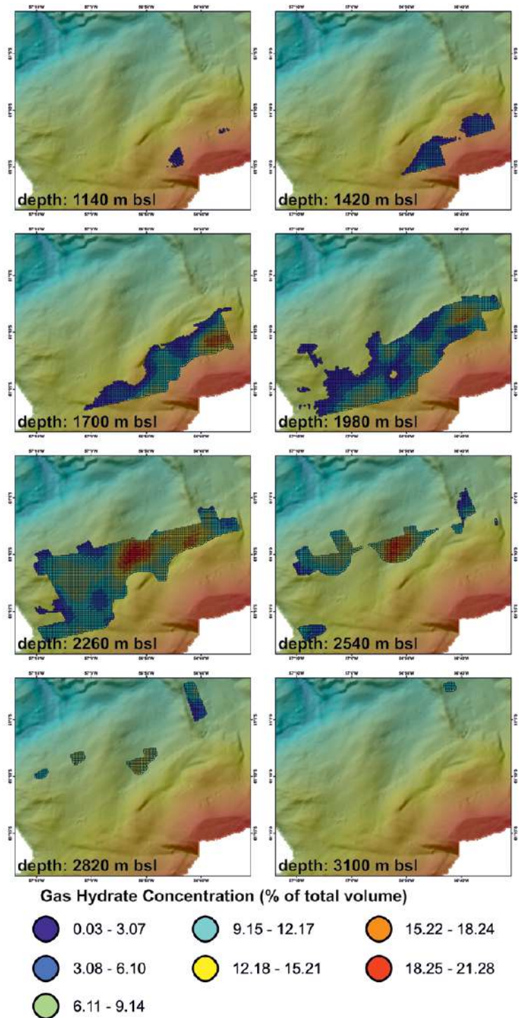
Figure 7. Map of the gas hydrate concentrations at different depth from seafloor (in meters).
