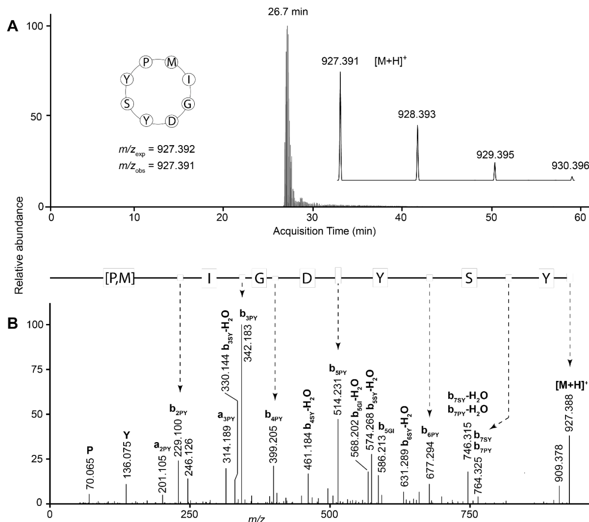
Figure S3. LC-MS data for anomuricin G with sequence cyclo-MIGDYSYP. (A) Extracted ion chromatogram showing acquisition time of the peptide, with (inset left) peptide sequence with expected and observed mass-to-charge ratios ( m/z ) and (inset right) peptide mass spectrum. (B) Tandem mass spectrum of the fragmented precursor ion. Immonium ions are denoted by the one-letter code of the residue they represent. The derived amino acid sequence is shown above the spectrum; residues in square brackets could not be assigned an order.
