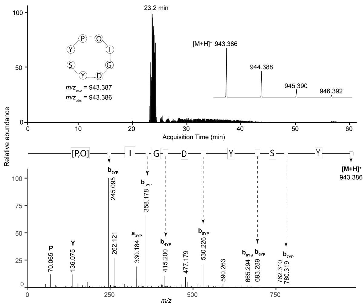
Figure S4. LC-MS data for anomuricatin G with sequence cyclo-MIGDYSYP, although the Met was oxidized (hence O in figure) (A) Extracted ion chromatogram showing acquisition time of the peptide, with (inset left) peptide sequence with expected and observed mass-to-charge ratios ( m/z ) and (inset right) peptide mass spectrum. (B) Tandem mass spectrum of the fragmented precursor ion. Immonium ions are denoted by the one-letter code of the residue they represent. The derived amino acid sequence is shown above the spectrum; residues in square brackets could not be assigned an order.
