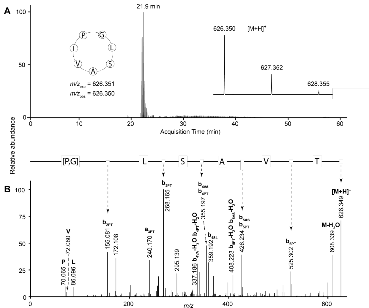
Figure S2. LC-MS data for anomuricatin F with sequence cyclo-GLSAVTP. (A) Extracted ion chromatogram showing acquisition time of the peptide, with (inset left) peptide sequence with expected and observed mass-to-charge ratios ( m/z ) and (inset right) peptide mass spectrum. (B) Tandem mass spectrum of the fragmented precursor ion. Immonium ions are denoted by the one-letter code of the residue they represent. The derived amino acid sequence is shown above the spectrum; residues in square brackets could not be assigned an order.
