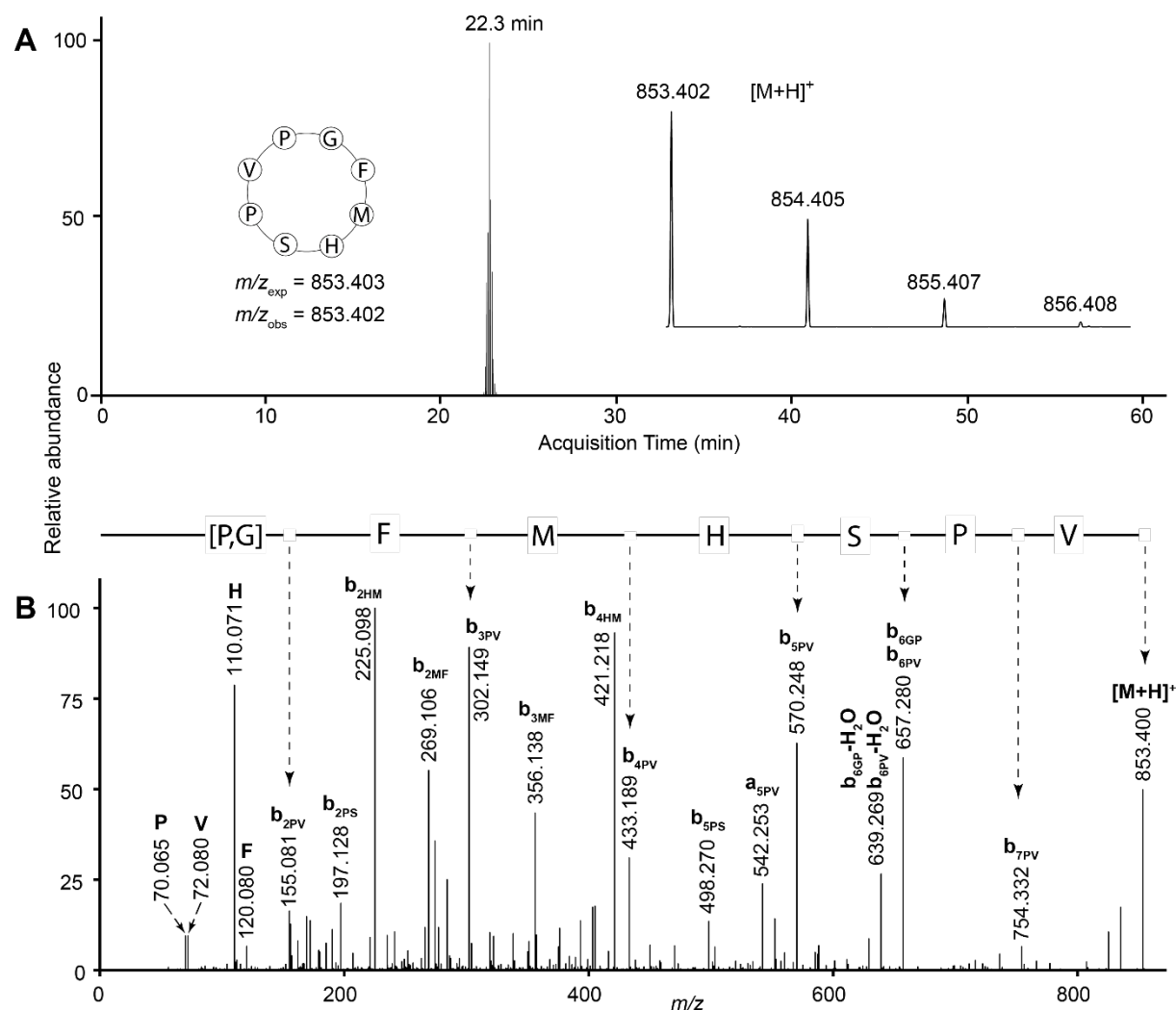
Figure S6. LC-MS data for anomuricin I with sequence cyclo-GFMHSPVP. (A) Extracted ion chromatogram showing acquisition time of the peptide, with (inset left) peptide sequence with expected and observed mass-to-charge ratios ( m/z ) and (inset right) peptide mass spectrum. (B) Tandem mass spectrum of the fragmented precursor ion. Immonium ions are denoted by the one-letter code of the residue they represent. The derived amino acid sequence is shown above the spectrum; residues in square brackets could not be assigned an order.
