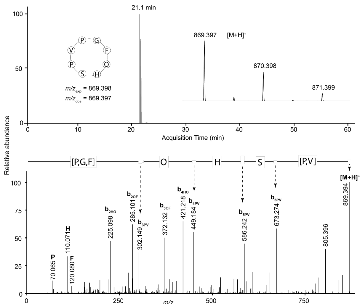
Figure S7. LC-MS data for anomuricatin I with sequence cyclo-GFMHSPVP, although the Met was oxidized (hence O in figure). (A) Extracted ion chromatogram showing acquisition time of the peptide, with (inset left) peptide sequence with expected and observed mass-to-charge ratios ( m/z ) and (inset right) peptide mass spectrum. (B) Tandem mass spectrum of the fragmented precursor ion. Immonium ions are denoted by the one-letter code of the residue they represent. The derived amino acid sequence is shown above the spectrum; residues in square brackets could not be assigned an order.
