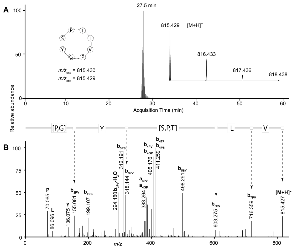
Figure S5. LC-MS data for anomuricin H with sequence cyclo-TLVPGYSP. (A) Extracted ion chromatogram showing acquisition time of the peptide, with (inset left) peptide sequence with expected and observed mass-to-charge ratios ( m/z ) and (inset right) peptide mass spectrum. (B) Tandem mass spectrum of the fragmented precursor ion. Immonium ions are denoted by the one-letter code of the residue they represent. The derived amino acid sequence is shown above the spectrum; residues in square brackets could not be assigned an order.
