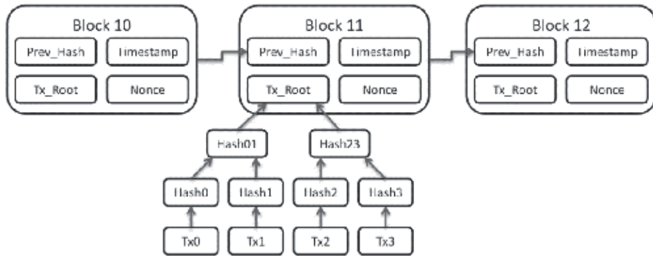
Figure 2. Merkle tree.
