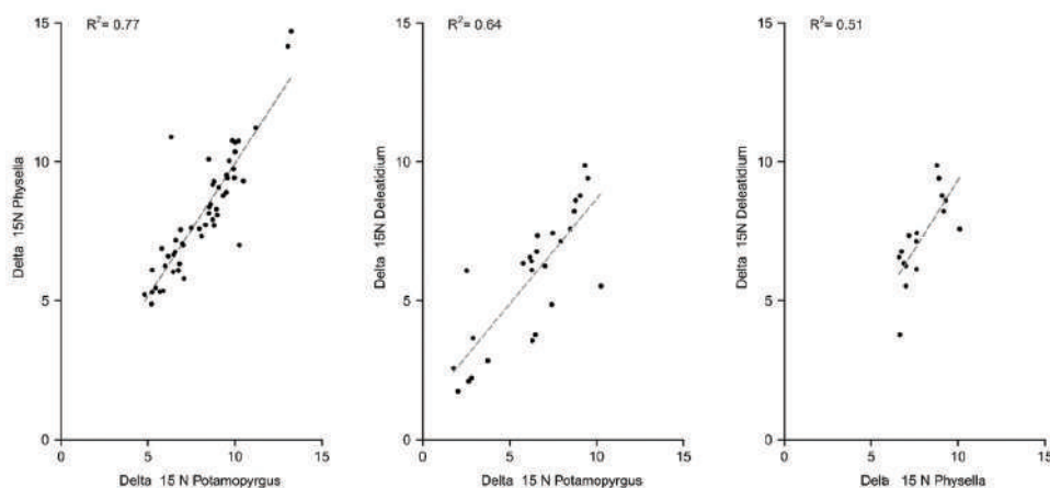
Figure 3. Comparison of primary consumers \delta^{15}\text{N} ratios at stream sites where more than one grazer taxon occurred. The fitted linear regressions between taxa \delta^{15}\text{N} values are represented by the dashed lines and the strength of the relationships by the R^2 values.
