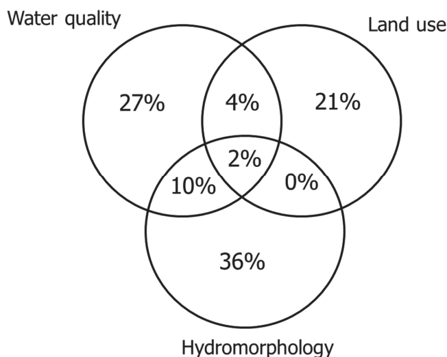
Figure 3. Venn diagram representing stressor-specific and joint effect contributions of the stressor variable groups to the explained variability of the benthic invertebrate assemblages. Explained variability is given as percentage of the total explained variance.
