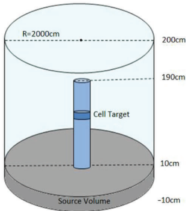
Figure 1. MC geometry model of the MCNP6.1 simulation including the source, the phantom and all the patterns used in it. The whole setting is as follows: the human phantom (depicted as a blue thin cylinder of 1.80 m height and 25 cm radius) stands in the middle of the outer azure cylinder (radius 20 m) which is filled with air (surrounding environment). The grey base cylinder (radius 20 m) represents the source volume on which the “human” stands (i.e., the surrounding ground, composed of soil and contaminated with the radionuclide ^{137}\text{Cs} in different surface activity values). There is no proportionality in the depicted dimensions of the patterns for the sake of simplicity.
