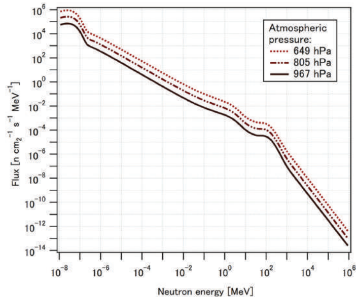
Figure 6. The neutron-energy spectra calculated by the model PARMA [18,19] at three locations along the route (indicated with red points in Figure 1) in the period from December 2018 to January 2019.
