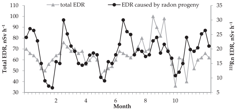
Figure 3. Variations of the equivalent dose rate caused by ^{222}\text{Rn} and total equivalent dose rate in the underground parking lots.
