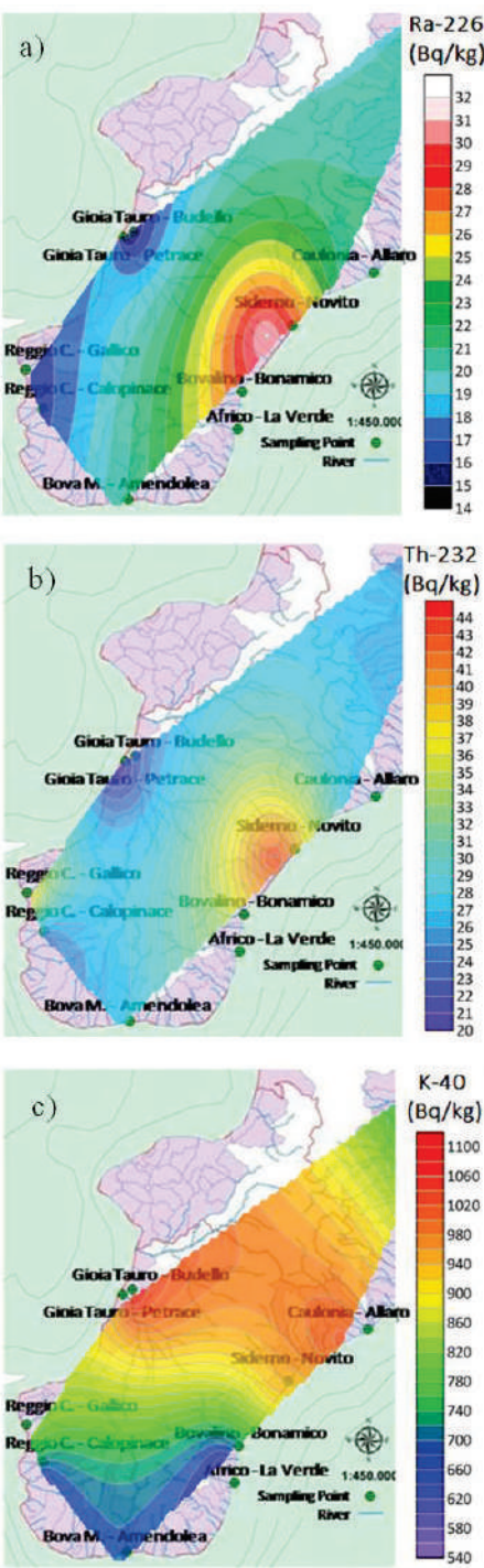
Figure 2. Contour maps showing the spatial distributions of (a) ^{226}\text{Ra} , (b) ^{232}\text{Th} and (c) ^{40}\text{K} in the investigated region.
