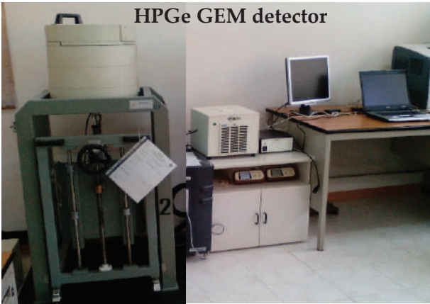
Figure 2. HPGe gamma spectrometry setup.
