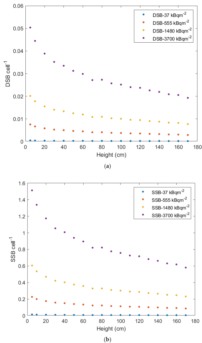
Figure 3. Estimation of the number of (a) DSBs and (b) SSBs per cell, respectively, induced by different levels of 137 Cs contamination in the ground, for the exposure time of one week, according to our MCDS simulations.
