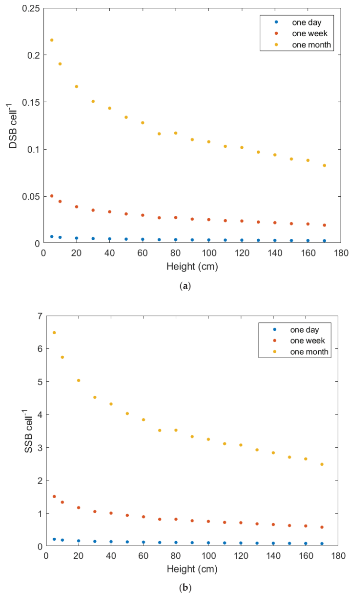
Figure 5. Estimation of the number of (a) DSBs and (b) SSBs per cell, formed by dose induced by a ^{137}\text{Cs} ionizing radiation of surface activity 3700 \text{ kBq}\cdot\text{m}^{-2} for an exposure time of a day, one week and a month, using MCDS simulations.
