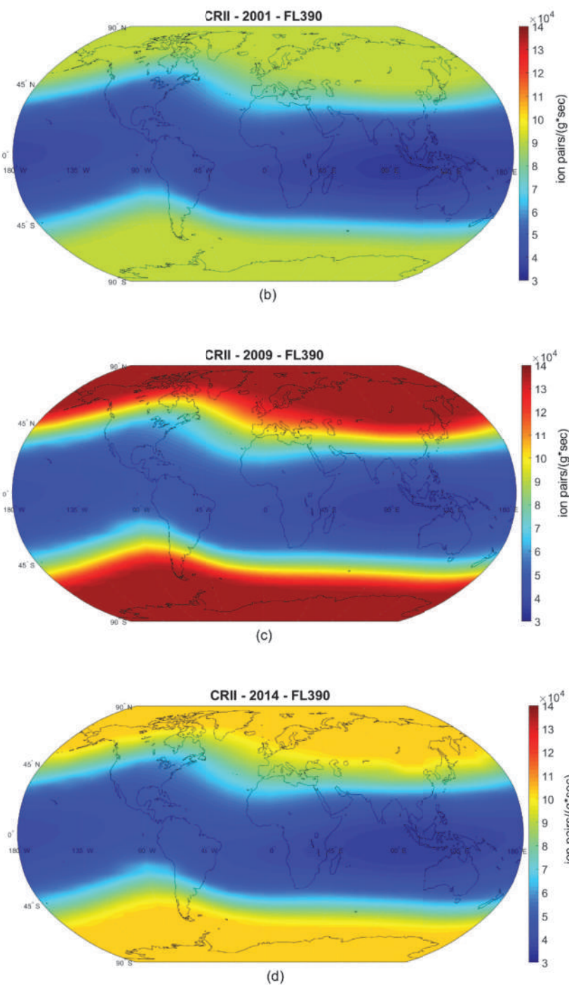
Figure 1. Maps of the CRII rate (ion pairs/(g*s)) at FL390: (a) during the minimum of solar cycle 23; (b) during the maximum of solar cycle 23; (c) during the minimum of solar cycle 24; (d) during the maximum of solar cycle 24.
