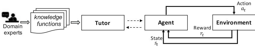
Fig. 1 Overall Working of Tutor4RL
