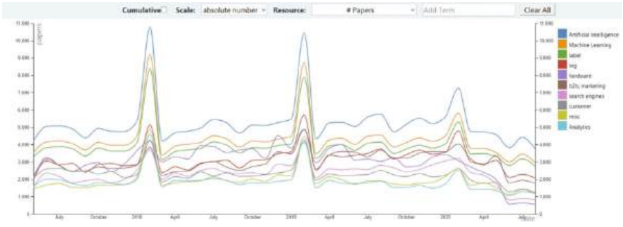
Fig. 16 Time series (Topics, accessed in November 2020)
