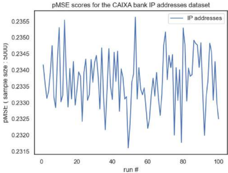
Fig. 4 Results for 100 random sampling taken from the real and synthetic data (5 K datapoints each) and the pMSE calculated using a logistic model
