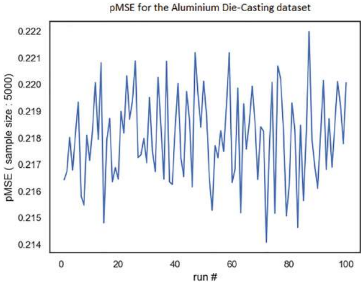
Fig. 5 Results for 100 random sampling taken from the real and the synthetic data (5K datapoints each) and the pMSE calculated using a logistic model
