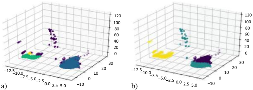
Fig. 6 (a) DBSCAN representation. (b) K -means representation
