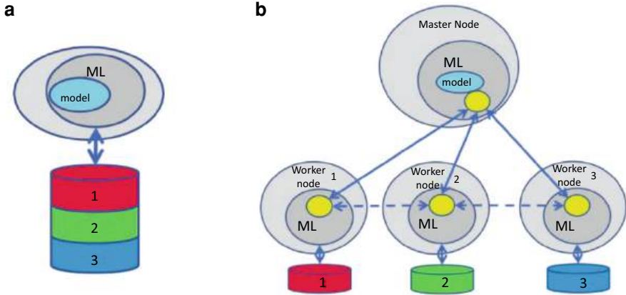
Fig. 2 Centralized approach (a) vs our privacy-preserving distributed scenario (b) where every user provides a portion of the training set
