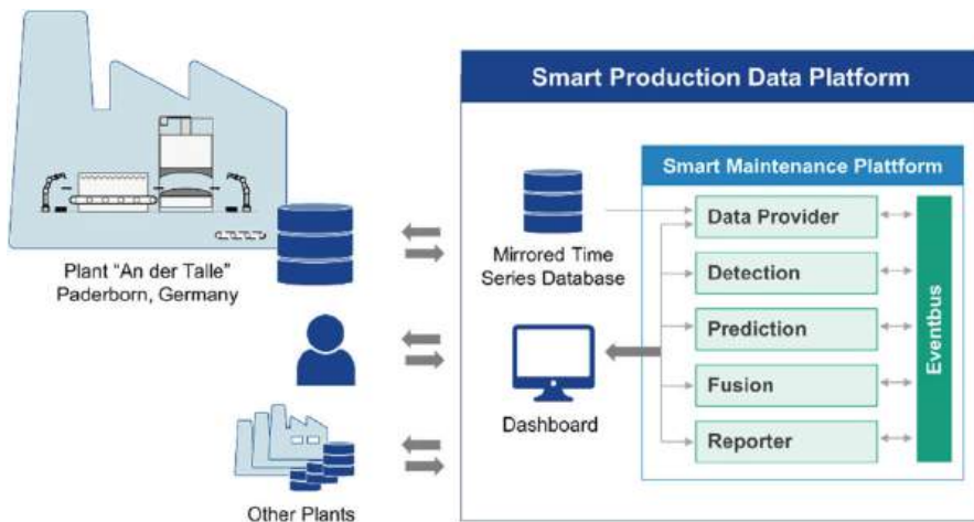
Fig. 9 Production data platform: A Smart Maintenance service accesses the provided data, uses modules for data analysis and visualizes the results in a dashboard (source: IEM/ATLANTIS Engineering)
