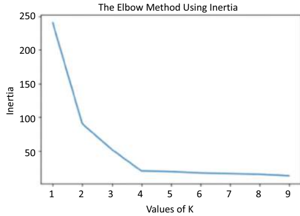
Fig. 8 Number of clusters selection for ‘Enhanced control of customers in online banking’
