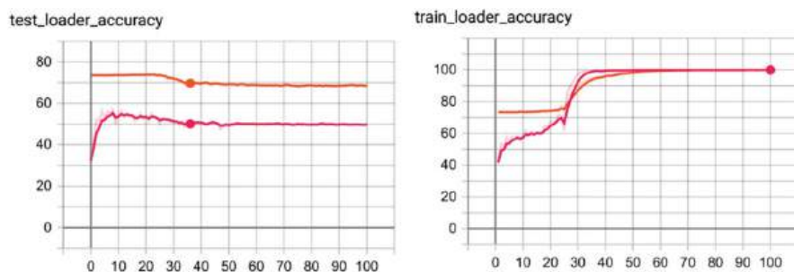
Fig. 4 Training and testing accuracy for the two joint neural network models: when trained on full imbalanced data (orange line) and when trained on sub-sampled balanced data (pink line)
