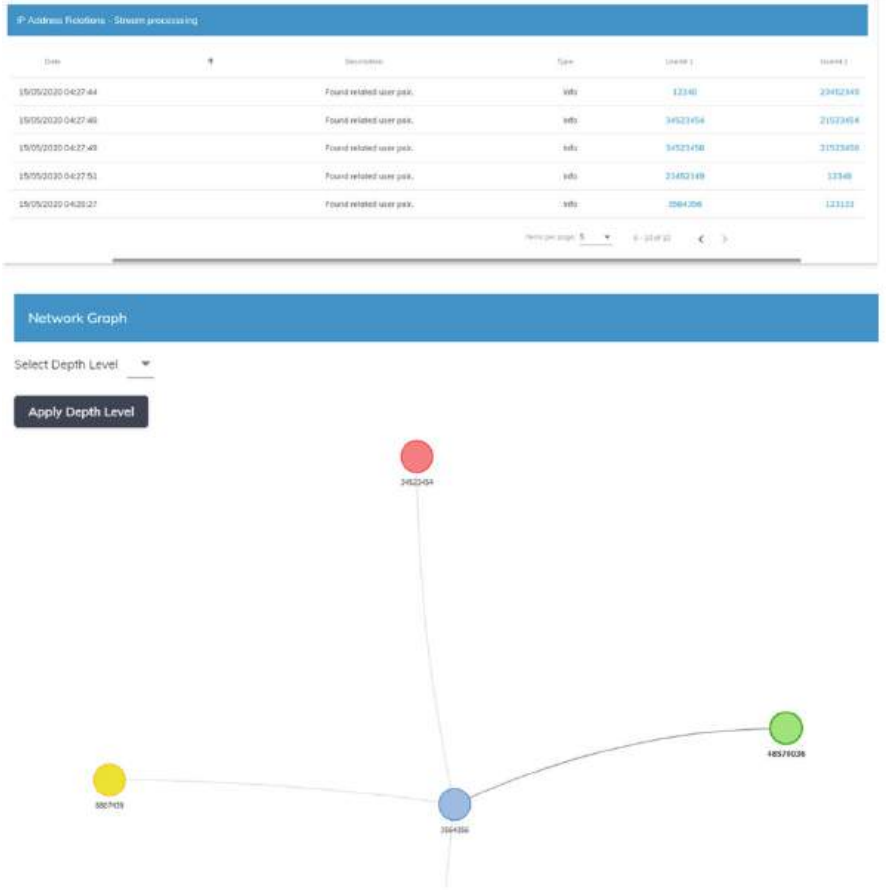
Fig. 3 (a) User groups per IP relationships. (b) Real-time relationship detection
