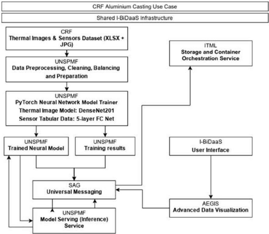
Fig. 2 Architecture of the ‘production process of aluminium die-casting’ use case
