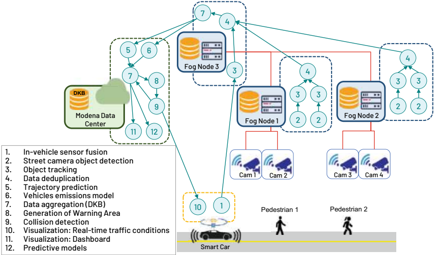
Fig. 8 Example of big data analytics distribution on the MASA and vehicles infrastructure
