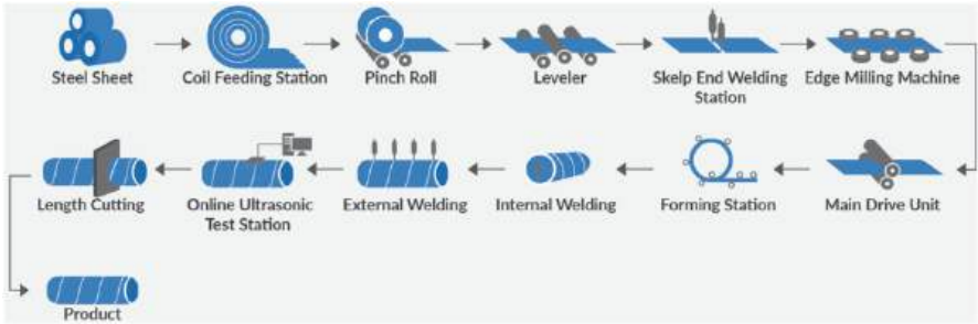
Fig. 3 Spiral welded steel pipe process
