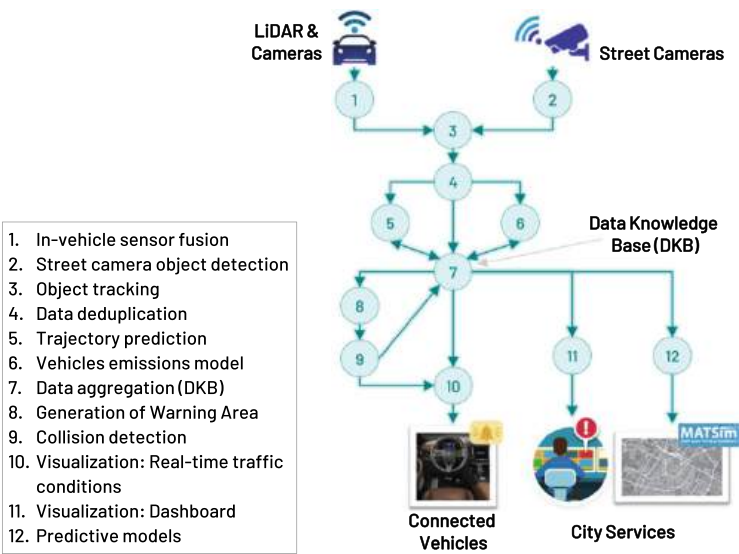
Fig. 5 Integration of the big data analytics
