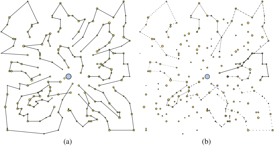
Fig. 8.3 (a) The optimal solution to a VRP instance. (b) A few tours quickly obtained with a taboo search. We notice great similarities between the latter and those of the optimal solution
