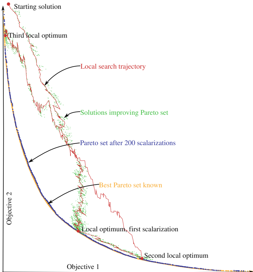
Fig. 5.12 Trajectory and evolution of an iterated local search for the bi-objective TSP instance (EuclidAB100) using the scalarization technique. The improvement method is based on an ejection chain. The weights associated with the objectives are randomly drawn each time the search reaches a local optimum. The starting solution is obtained by a greedy constructive method working solely on the first objective
