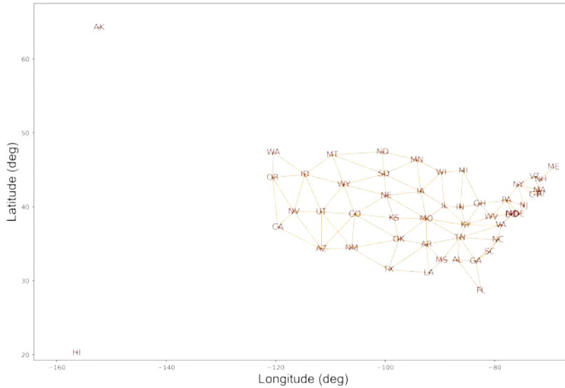
Figure 12.10: Graph representation of the 51 states forming the United States of America in Example 12.5.
