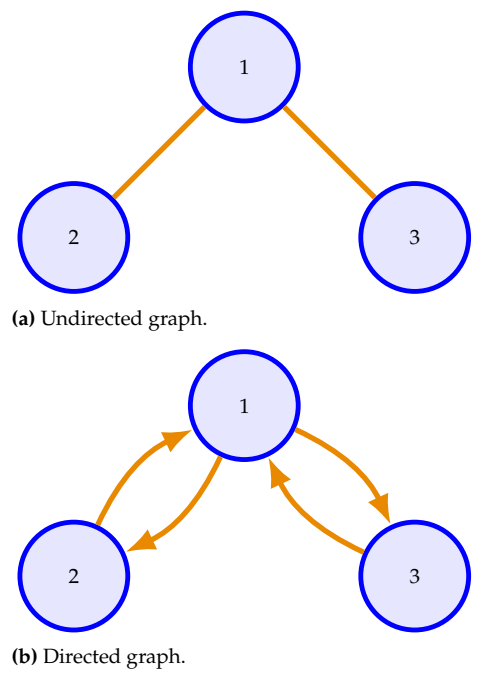
Figure 11.4: Example of undirected graph and its transformation into a directed graph. Note: we assumed that every (v_1, v_2) edge of the undirected version was replaced by both edge (v_1, v_2) and edge (v_2, v_1) in the directed version.
