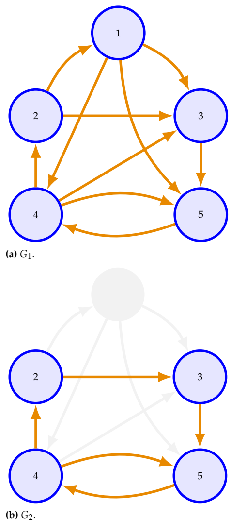
Figure 11.5: A directed graph G_1 and a subgraph G_2 of G_1 . In Figure 11.5b we highlight with light gray the vertices and edges that were removed from G_1 to obtain subgraph G_2 .
