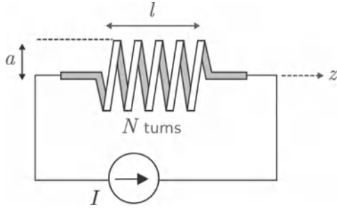
Figure 7.6: Determination of the magnetic field due to DC current in a coil.
