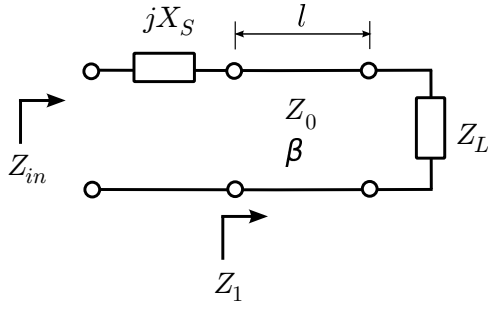
Figure 3.28: Single-reactance matching with a series reactance.
