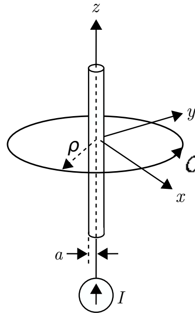
Figure 7.3: Determination of the magnetic field due to steady current in an infinitely-long straight wire.
