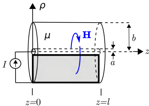
Figure 7.18: Determining the inductance of coaxial line.
