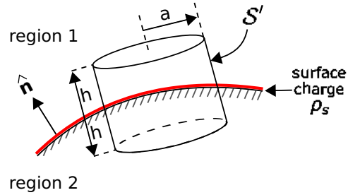
Figure 5.10: Use of Gauss' Law to determine the boundary condition on \mathbf{D} .
