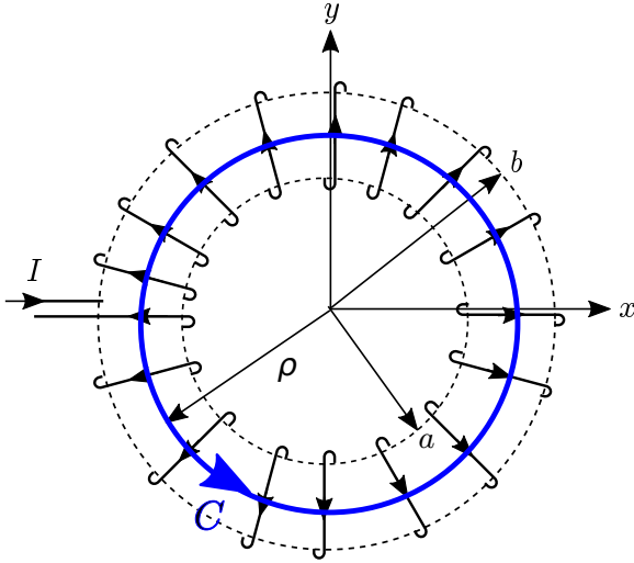
Figure 7.12: Selected path of integration.
