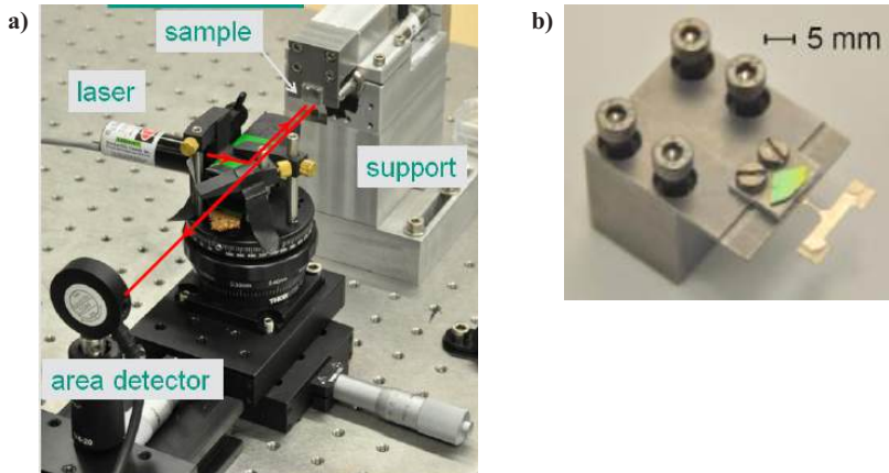
Fig. 5.3. a) Test setup for HCF experiments on micro-samples, measurement of the sample displacements via laser beam, b) micro-sample fixed in the clamp [85].
