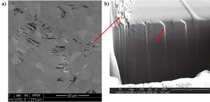
Fig. 5.15. Surface inspection of a Ni-sample after an HCF experiment ( 4 \times 10^6 cycles of uniaxial reversed bending with an amplitude of \pm 200 MPa): a) SEM micrograph of grains exhibiting micro-damage (extrusions and intrusions), b) FIB cross section of a damaged grain showing a micro-crack initiated from surface protrusions.
