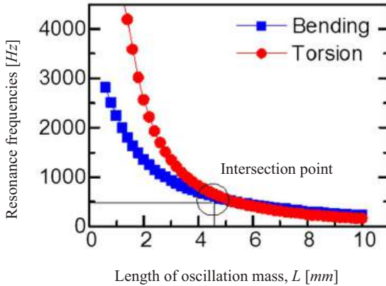
Fig. 5.9. Optimization of length L for equal resonance frequencies at bending and torsion modes. Reference of the diagram is [86], with some small modifications.
