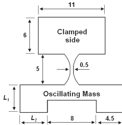
Fig. 5.8. Optimized geometry of micro-samples for multiaxial HCF tests. Dimensions are in [mm]. L_1=L_2=4.5 mm. References for the drawing and geometrical data of the samples are [85, 88], with some small modifications.
