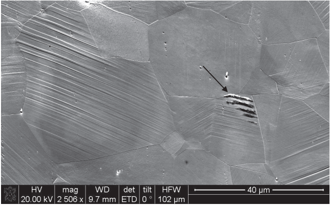
Fig. 6.16. Regular surface markings due to dislocations along slip bands. Formation of PSBs in one grain due to strain localization, sample No. Ni-105 (after 10^7 cycles of uniaxial bending with an amplitude of \pm 150 MPa).
