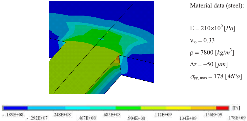
Fig. 5.5. Model with non-optimized sharp corners: bending stress at the shoulder due to a vertical displacement of 50 \mu m (at the free end of the twin inertial masses).
