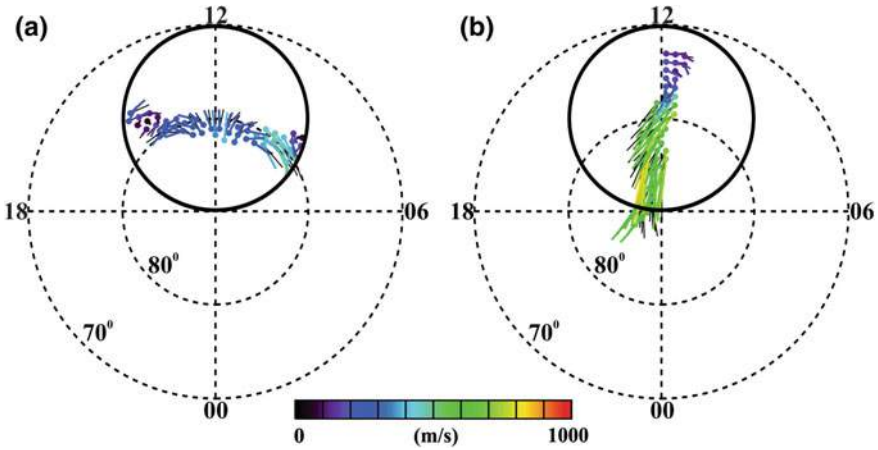
Fig. 9.8 Coloured vectors indicate convection calculated for \theta_c = 10^\circ and K_{max} = 3 for a spherical cap centred at 70° MLAT and 12 MLT for Swarm A and C measurements artificially generated using the a IMF B_z > 0 convection pattern for a Swarm A satellite track offset 80° from the 12 MLT meridian and p = 12 and b IMF B_z < 0 convection pattern for a Swarm A satellite track offset 170° from the 12 MLT meridian and p = 12 . Black vectors in (a) and (b) indicate the direction of the statistical model convection
