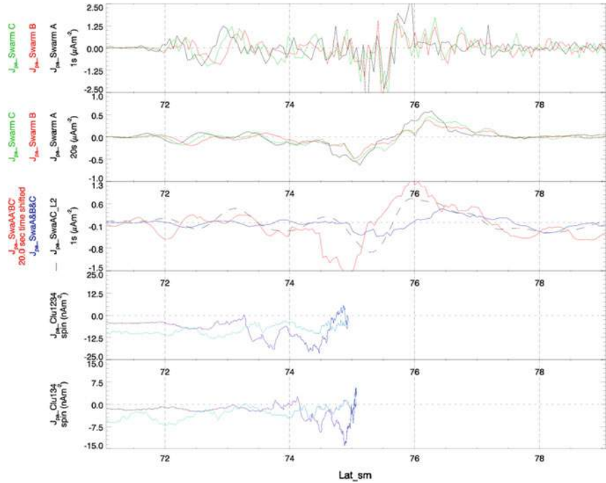
Fig. 5.13 Plot taken from Dunlop et al. (2015b), showing the mapped MLAT values (in SM coordinates) of Swarm and Cluster FACs. The top three panels correspond to the same set of FAC estimates as shown in the top set of panels in Fig. 4.3. The bottom two panels show Cluster FACs estimated by the full curlometer and from the face formed by C1, C3, C4 (which is almost perpendicular to the magnetic field), respectively. The light blue trace corresponds to the track of Cluster after the conjunction as it moves to lower latitudes, but far in local time from the Swarm track
