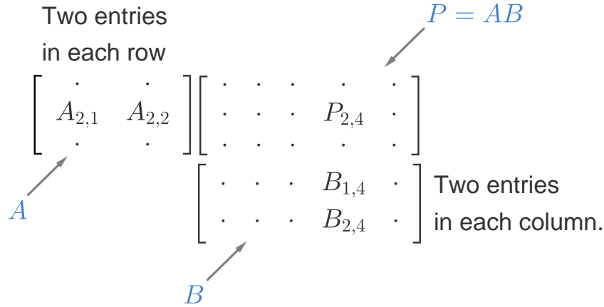
Figure 1.3.1: (AB)_{2,4} = P_{2,4} = A_{2,1}B_{1,4} + A_{2,2}B_{2,4}
