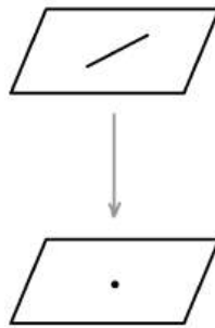
FIGURE 10.3. A first example of a blow-up
