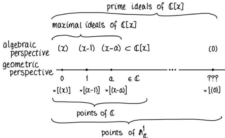
FIGURE 3.1. A picture of \mathbb{A}_{\mathbb{C}}^1 = \operatorname{Spec} \mathbb{C}[x]
