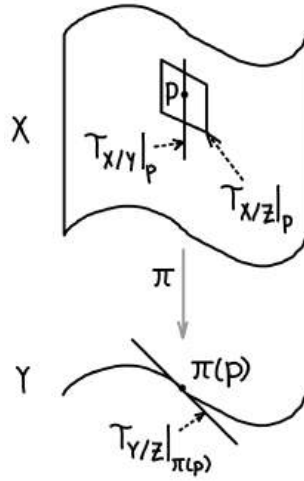
FIGURE 21.2. The geometry behind the cotangent exact sequence
