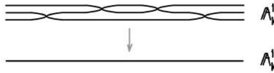
FIGURE 8.2. The “branched cover” \mathbb{A}_k^1 \rightarrow \mathbb{A}_k^1 of the “ u -line” by the “ t -line” given by u \mapsto p(t) is finite
