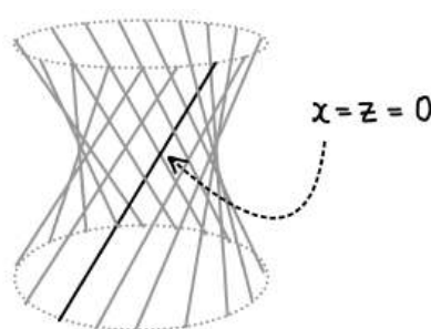
FIGURE 13.2. The line V(x, z) on the smooth quadric surface V(wz - xy) \subset \mathbb{P}^3 .
