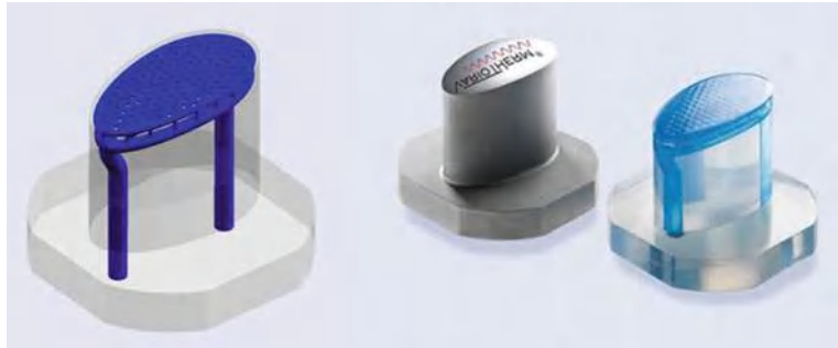
Fig. 6.37 Mesh surface for efficient mould insert cooling (Courtesy of GE Additive/Concept Laser)
