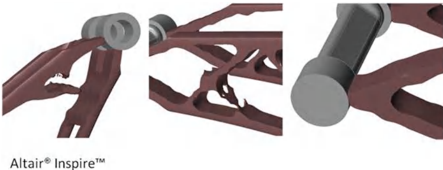
Fig. 5.15 Optimization issues ( https://community.altair.com/community ) (Courtesy of Altair)
