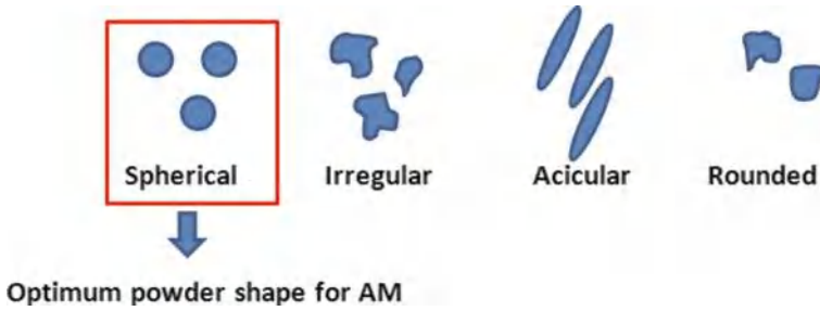
Fig. 7.15 Example of powder shapes (Source AIDIMME)
