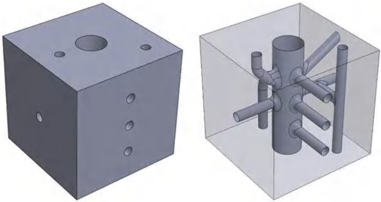
Fig. 4.1 Simplified ‘block’ design manifold with only the required in and out channels (Courtesy of Olaf Diegel [1])
