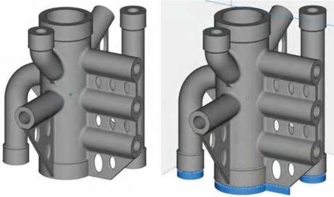
Fig. 4.4 Support material required by optimised for metal AM design (Courtesy of Olaf Diegel [1])
