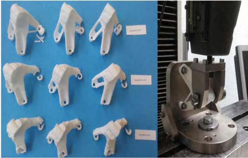
Fig. 5.23 SLS optimized parts in polyamide and mechanical testing ( Source Skin project—AIDIMME)
