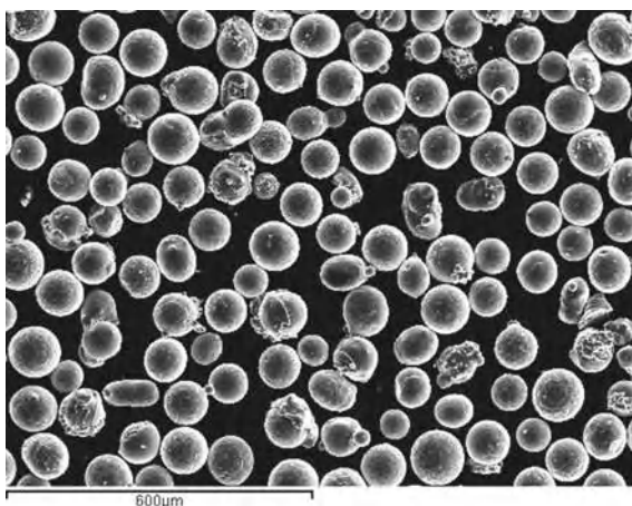
Fig. 7.16 TiAl powder particles produced by VIM (Source AIDIMME)
