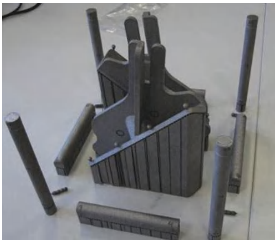
Fig. 7.35 Build cycle manufactured ( Source RepAir project, AIDIMME)
