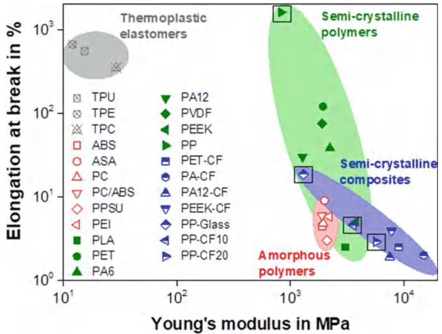
Fig. 7.2 Toughness/stiffness balance of MEX materials classified as thermoplastic elastomers, amorphous and semi-crystalline polymers, and semi-crystalline composites ([56]—licensed under CC BY)
