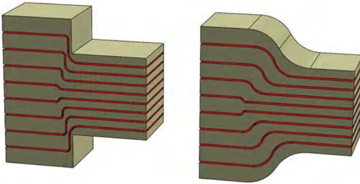
Fig. 4.21 Stress concentrations are the areas where cracks will most naturally form. Eliminating such stress concentrations can be critical to part quality (Courtesy of Olaf Diegel [1])
