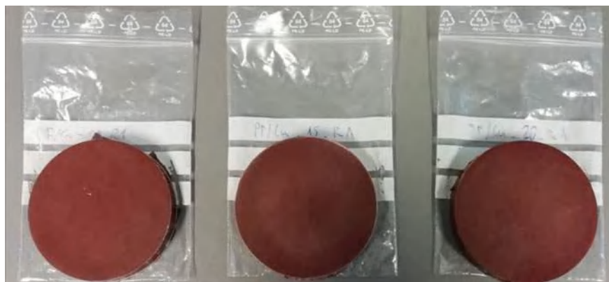
Fig. 7.11 Samples for thermal conductivity measurements prepared in the vacuum press (Source MUL facilities)
