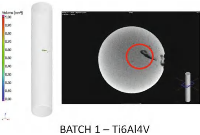
Fig. 7.47 Lack of fusion detection (Source Fractal project)
