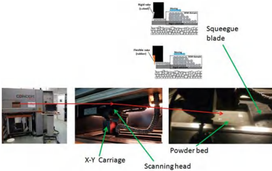
Fig. 1.19 PBF-LB/M overview ( Source AIDIMME facilities)
