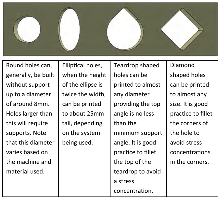
Fig. 4.23 Hole shapes that can be printed without the need for support material (Courtesy of Olaf Diegel [1])
