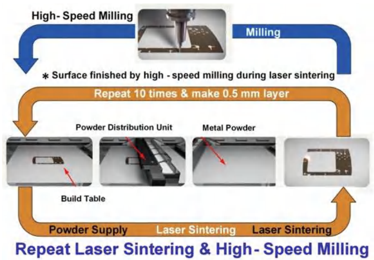
Fig. 6.21 Hybrid manufacturing process—PBF-LB/M (SLM) & HSC (Courtesy of Matsuura)
