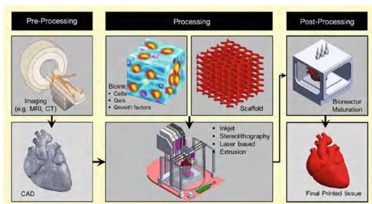
Fig. 6.69 Overview schematic of the bioprinting processes Copyright © 2021 Ramadan and Zourob [63], 648.—licensed under CC BY)
