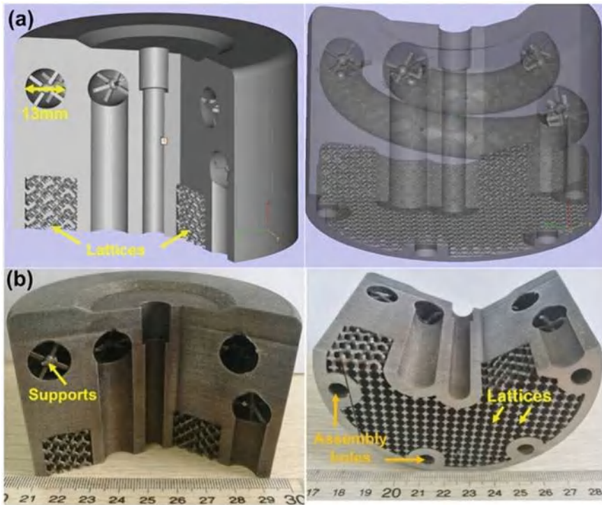
Fig. 6.34 Novel Conformal cooled mould insert: a CAD models of novel conformal cooled mould insert, b the corresponding mould insert processed by PBF-LB/M (Reprinted from Materials and Design, Vol. 196/109147, Chaolin et al. [10], Copyright 2021, with permission from Elsevier)
