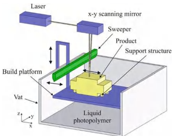
Fig. 1.5 Stereolithography (VPP-UVL/P) (Source Ana Pilipović)
