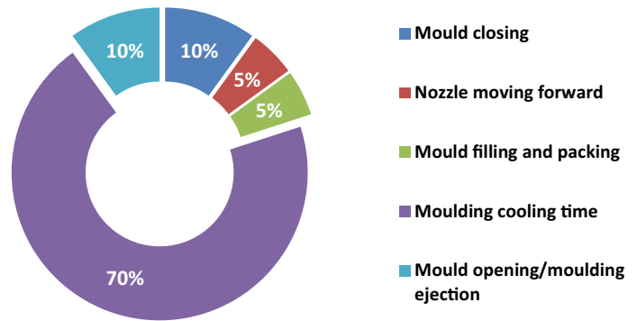
Fig. 6.25 Injection moulding cycle time analysis (Source Damir Godec)
