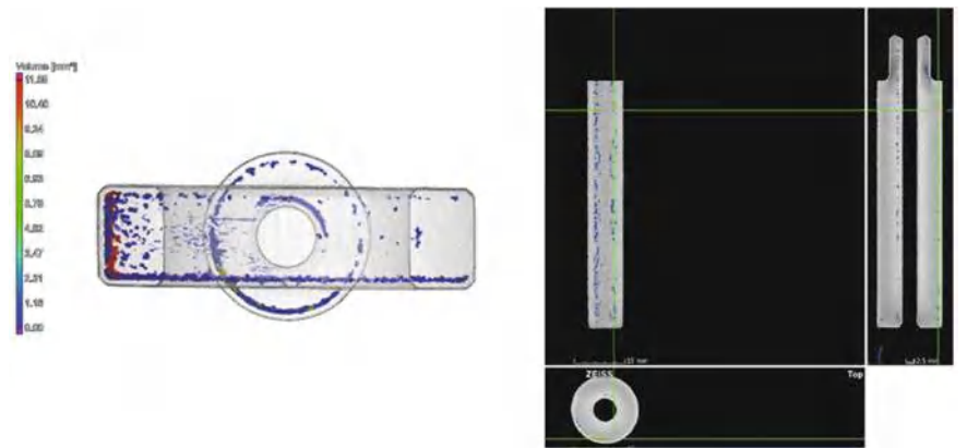
Fig. 7.49 Porosity detection in the borderline between contour and hatch due to wrong adjustment of overlap parameter ( Source Fractal project )
