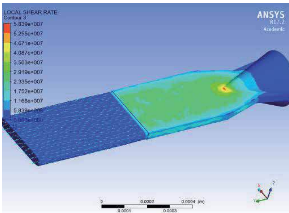
Figure 16. Distribution of shear deformations.
