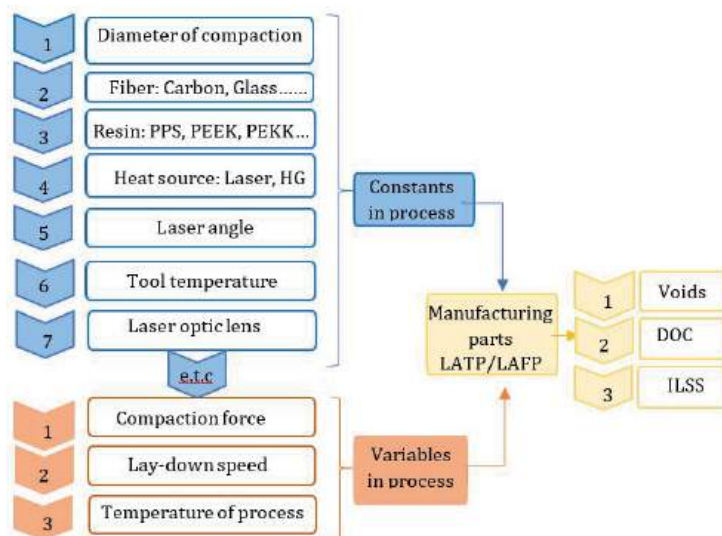
Figure 5. Constants and variables for the LATP process.
