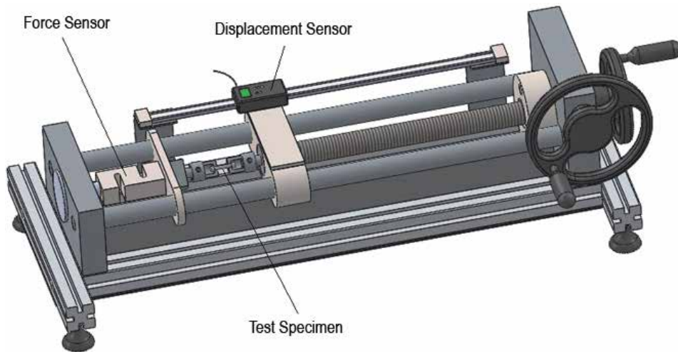
Figure 11. 3D CAD model of tensile testing machine.
