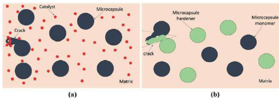
Figure 3. Schematic of capsuled-based mechanism: a) microcapsule/disperse catalyst system and b) dual capsuled-based system.
