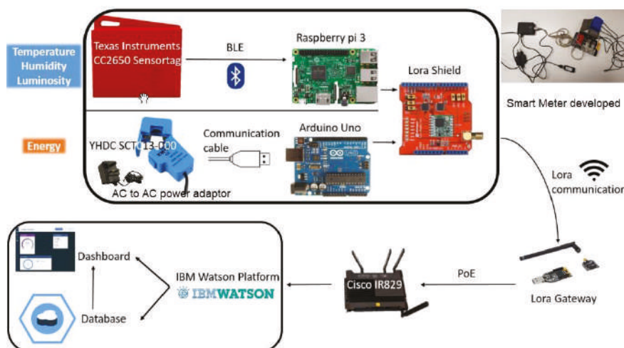
Figure 4. Smart meters for electricity measurement and a temperature/humidity sensor with a Lora network, sending data to IBM Watson.
