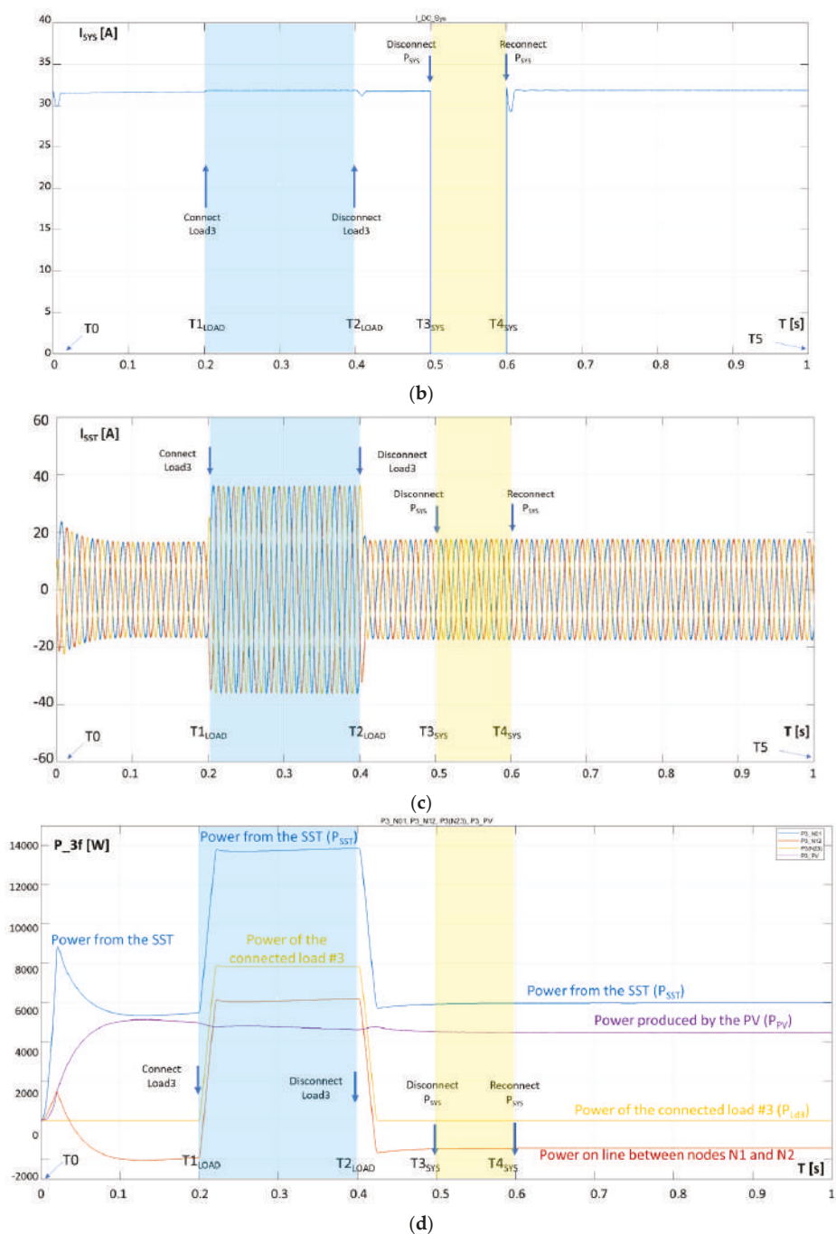
Figure 9. Simulation results in Scenario 2. (a) DC bus voltage in the SST; (b) Current injected from the main grid in the DC bus of the SST; (c) Output currents of the SST ( I_{SST} ), towards the microgrid (real-time values); (d) Active power evolution in different parts of the AC microgrid.
